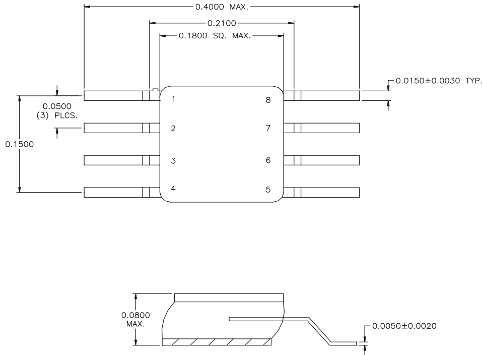
STANDARD CASE STYLE M47 (Optional Case Styles – M10)
