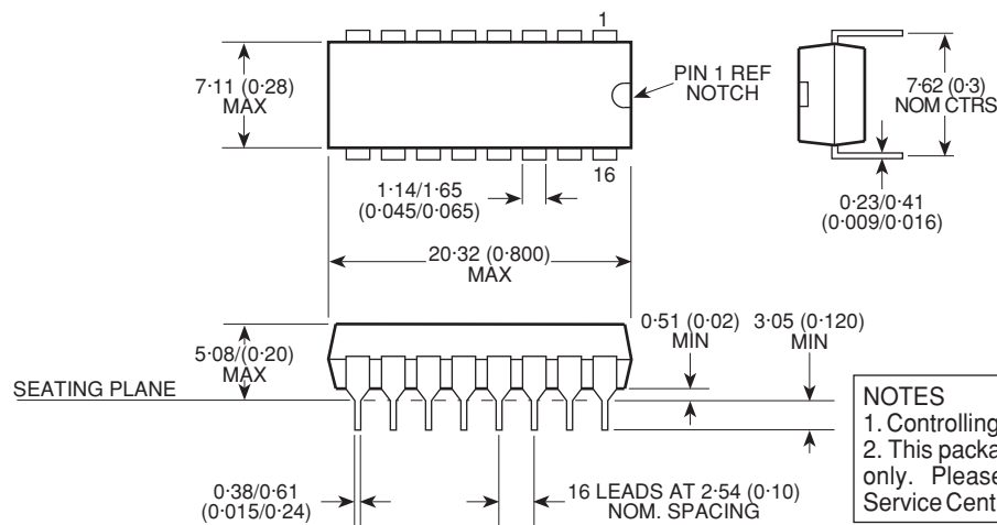
16-LEAD PLASTIC DIP – DP16
