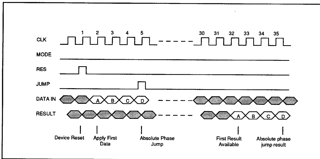
Fig. 9 Phase Modulation Timing Diagram
