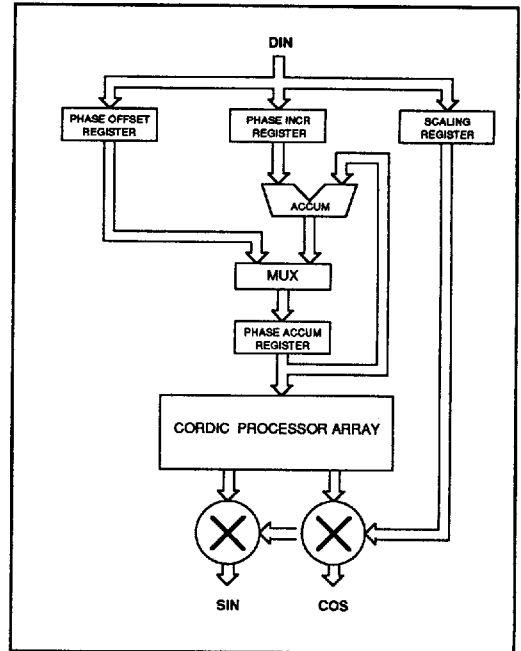
Fig. 1 Block Diagram
