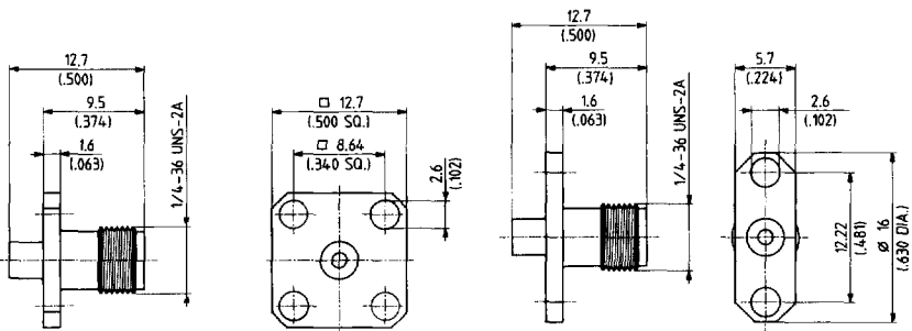
Fig. 1: square flange
