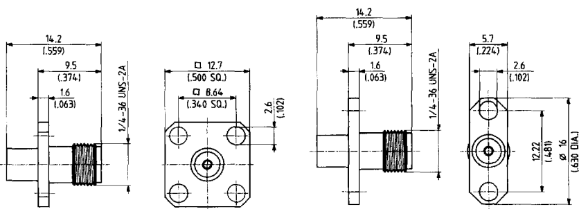
Fig. 1: square flange
