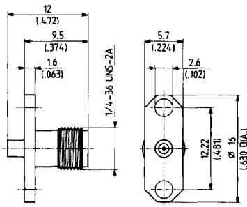
Fig. 2: 2-hole flange
