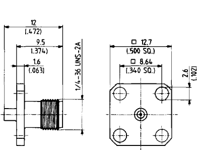
Fig. 1: square flange
