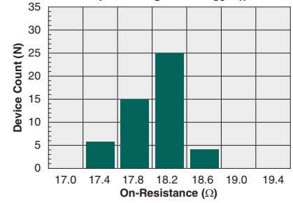
Typical On-Resistance Distribution (N=50, I_F=2\text{mA} , I_L=120\text{mA}_{\text{DC}} , T_A=25^\circ\text{C} )
