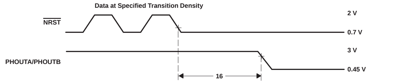
Figure 16. Watchdog-Timer Expiration Waveforms
