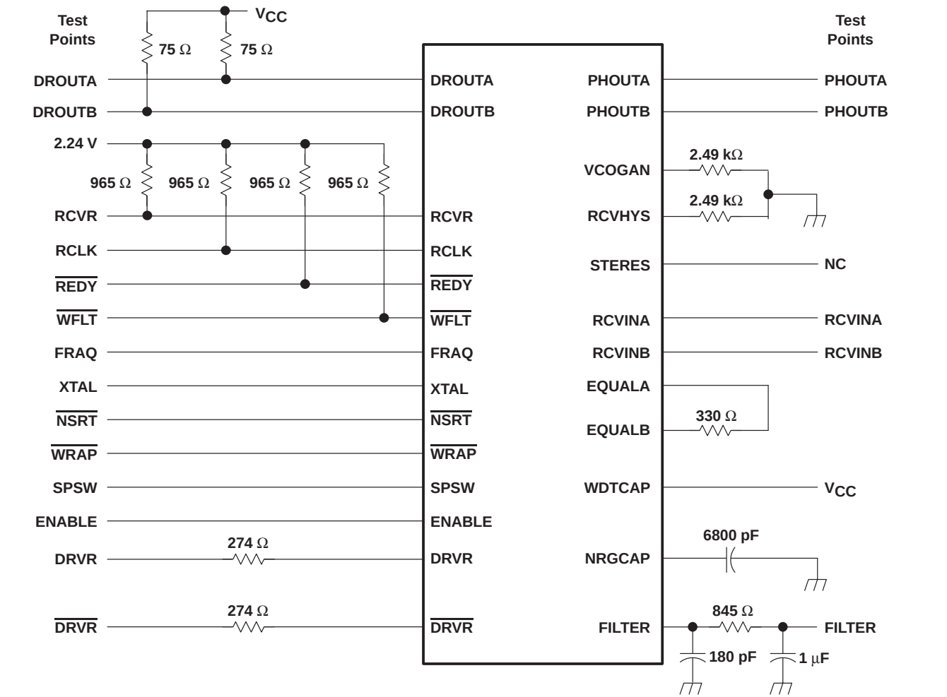
Figure 8. ac Test Circuit
