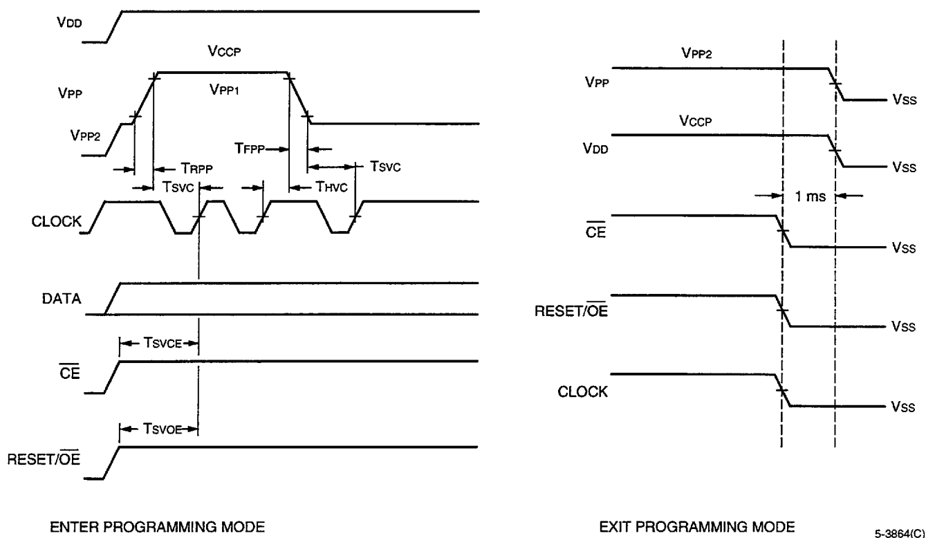
Figure 7. Entering and Exiting Programming Mode
