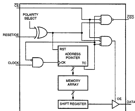
Figure 1. Block Diagram
