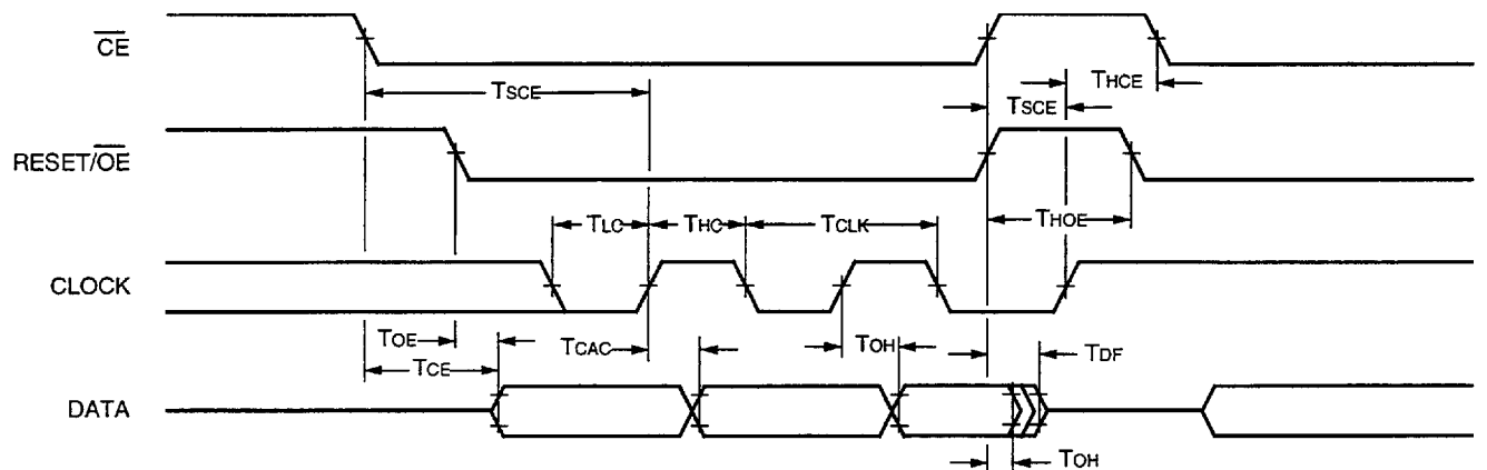
Figure 4. Read Characteristics
