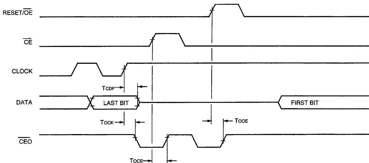
Figure 5. Read Characteristics at End of Array
