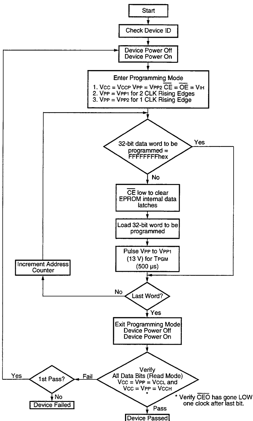
Figure 6. ATT1700A Programming
