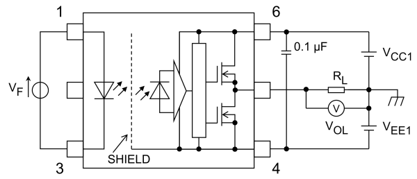
Fig. 13.1.4 V_{OL} Test Circuit
