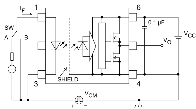
Fig. 13.1.8 Common-Mode Transient Immunity Test Circuit and Waveform
