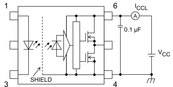
Fig. 13.1.6 I_{CCL} Test Circuit
