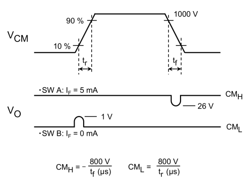
Fig. 13.1.8 Common-Mode Transient Immunity Test Circuit and Waveform
