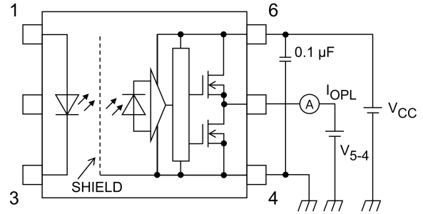
Fig. 13.1.2 I_{OPL} Test Circuit
