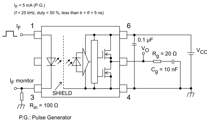
Fig. 13.1.7 Switching Time Test Circuit and Waveform
