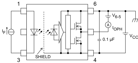
Fig. 13.1.1 I_{OPH} Test Circuit
