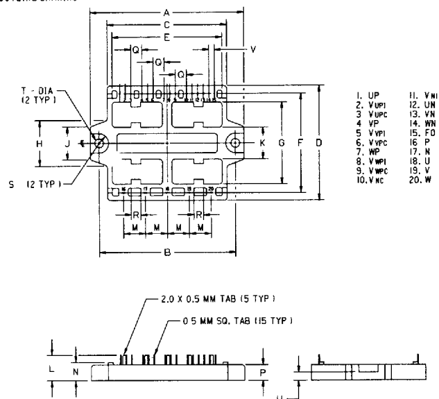
OUTLINE DRAWING
