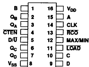
16-Lead Flatpack Top View
