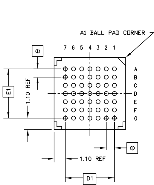
BOTTOM VIEW (49 SOLDER BALLS)
