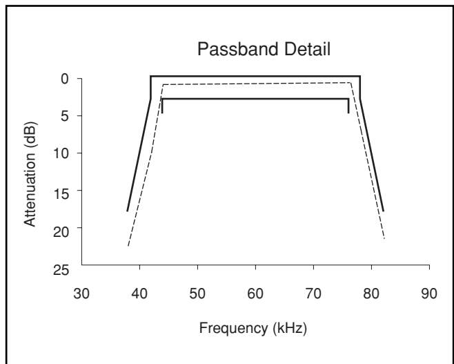
Figure 3 - Band Pass Filter Response
