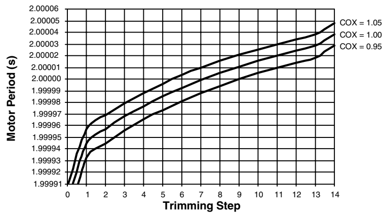
Figure 5-2. Typical Trimming Curve Characteristic for T_M of 2 s
