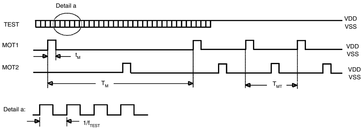
Figure 5-1. Motor Output Signal During Normal Operation and During Motor Test
