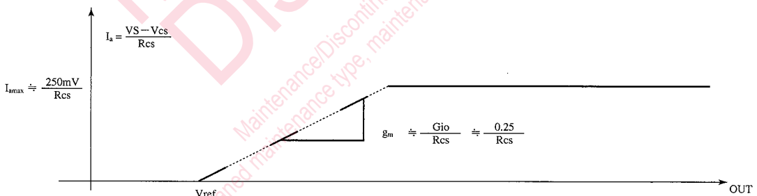
Fig.3 Drive Characteristics
