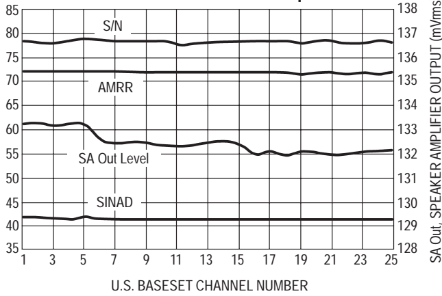
Figure 66. Typical Performance Parameters Over U.S. BaseSet Channel Frequencies
