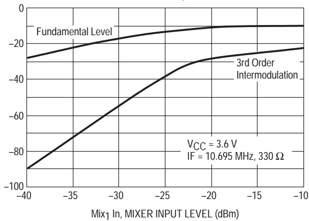
Figure 19. First Mixer Output Level and Intermodulation, IP3_bit = 0
