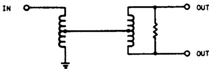
Functional Schematic
