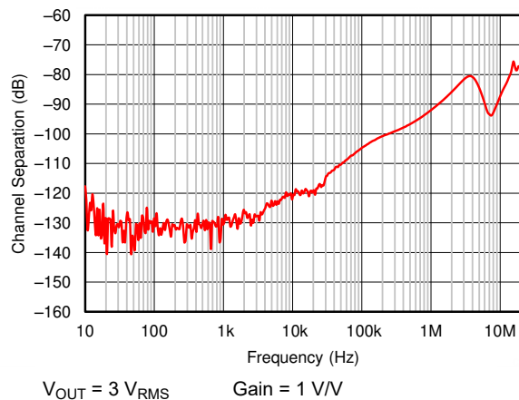
Figure 6-11. Channel Separation vs Frequency
