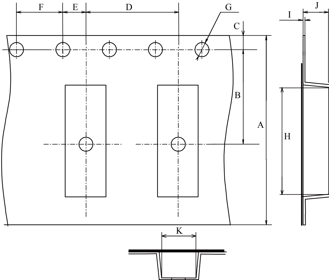
Dimension List
