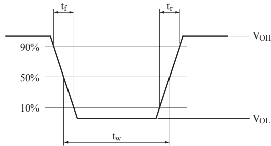
Fig.2 Output Waveform Specification(Receiver side)
