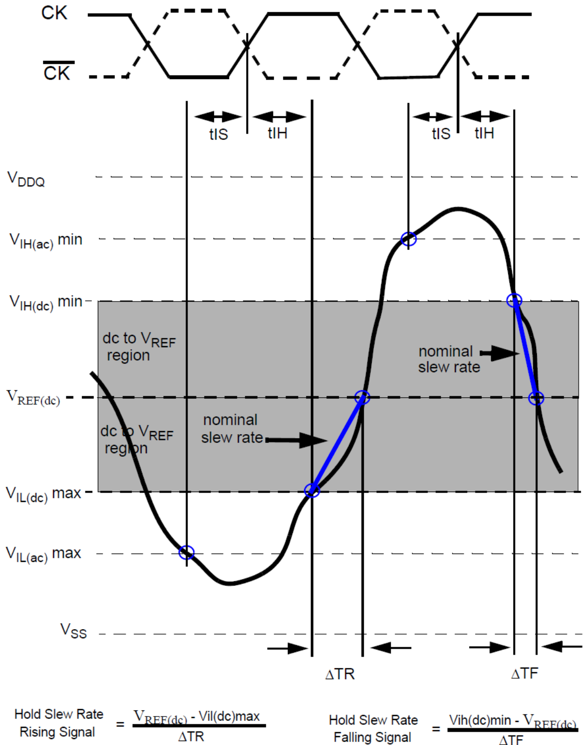
Illustration of nominal slew rate for tIH
