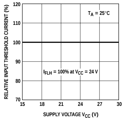
Figure 18. Normalized low to high threshold input current vs. supply voltage, HCPL-3101.
