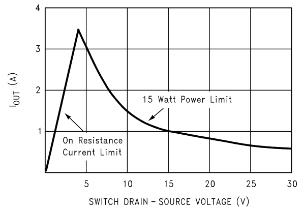
FIGURE 5. Maximum Output Current with Instantaneous Power Limiting
