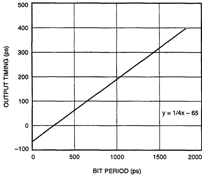
Figure 12. Data Clock Output Timing Diagram
