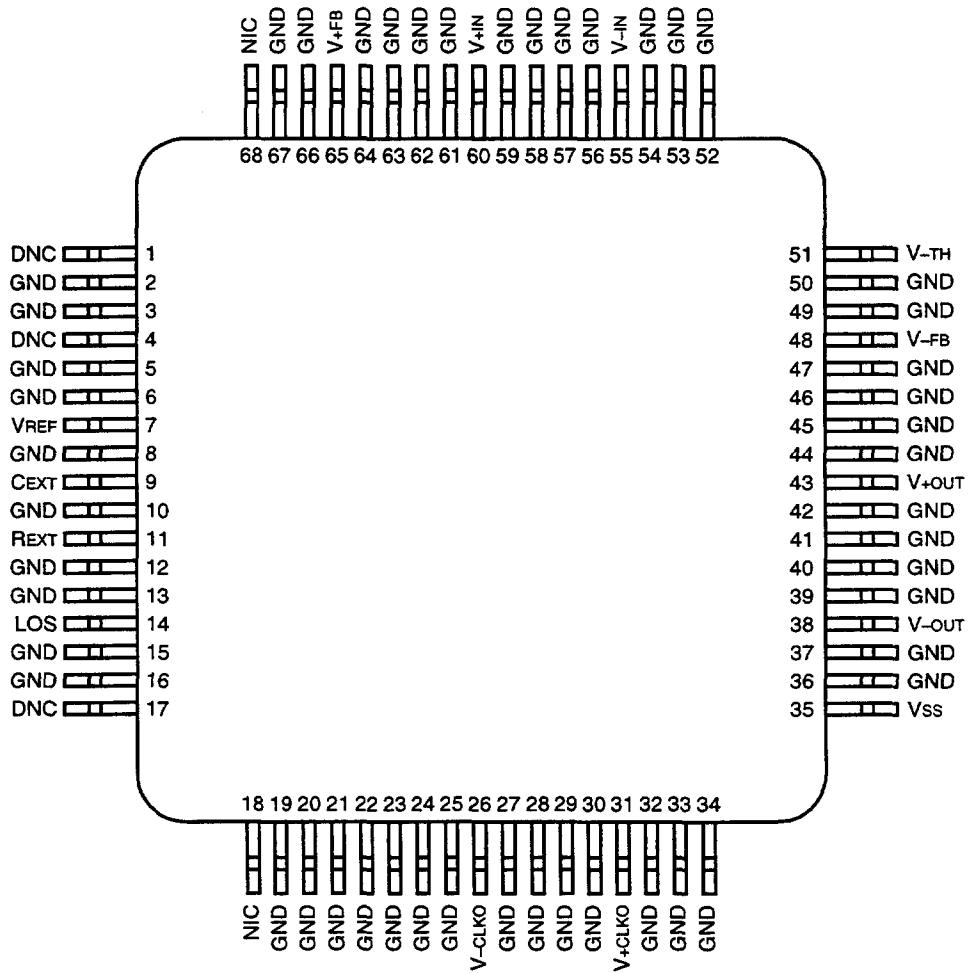
Figure 9. Pin Diagram
