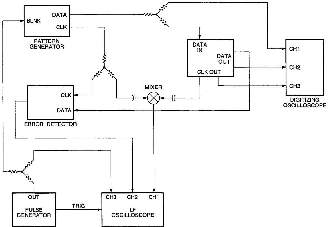
Figure 14. Error Recovery Test Circuit
