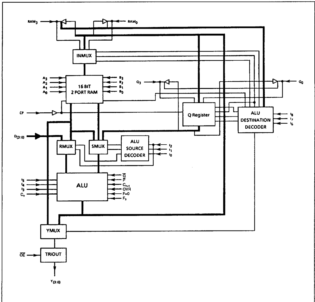
Figure 1: Block Diagram
