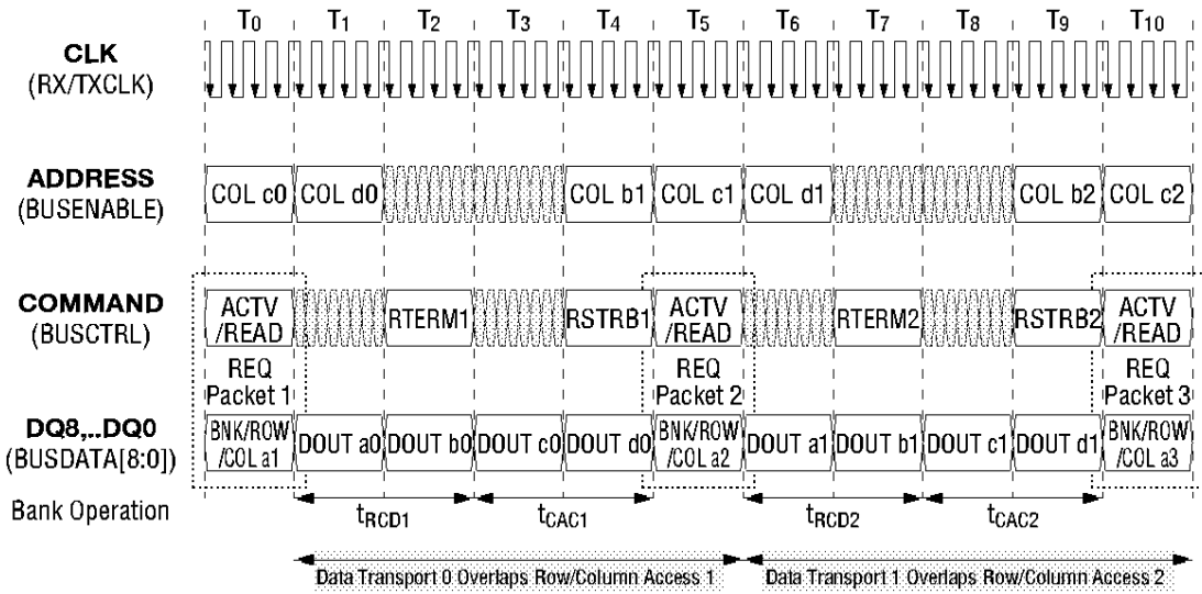
Fig. 5 Interleaved Read Transaction Example
