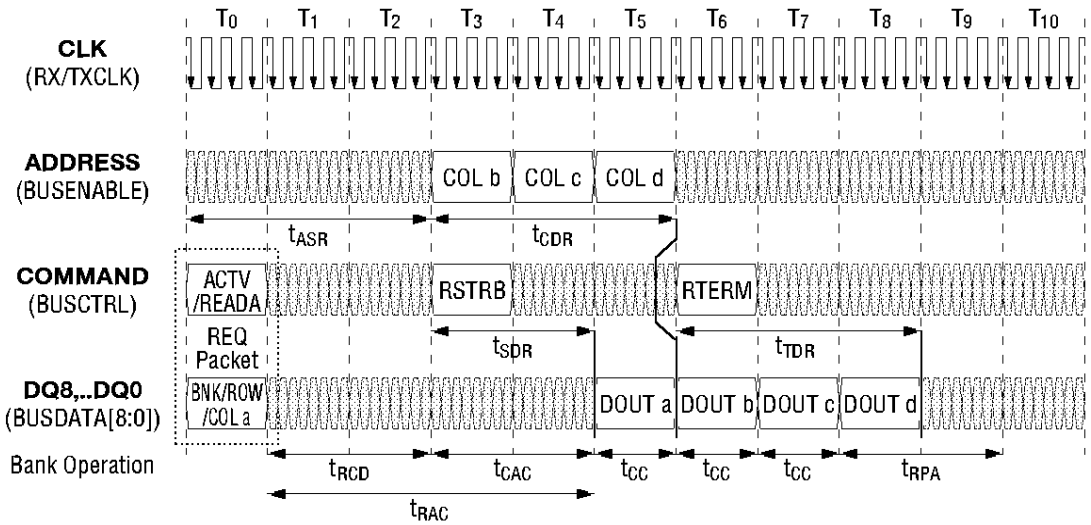
(b) ACTV/READA - BANK ACTIVATE AND RANDOM READ CYCLES WITHIN A PAGE
