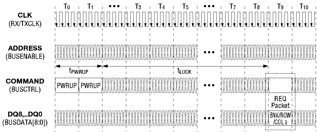
(c) PWRUP PACKET FOR POWERDOWN-TO-ENABLE POWER MODE TRANSITION
