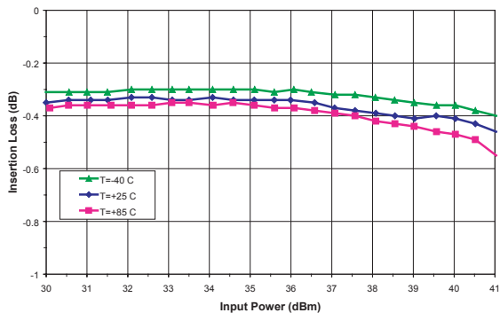
Figure 6: Compression vs. Temperature ( V_n = 3.0 V, F = 836 MHz)
