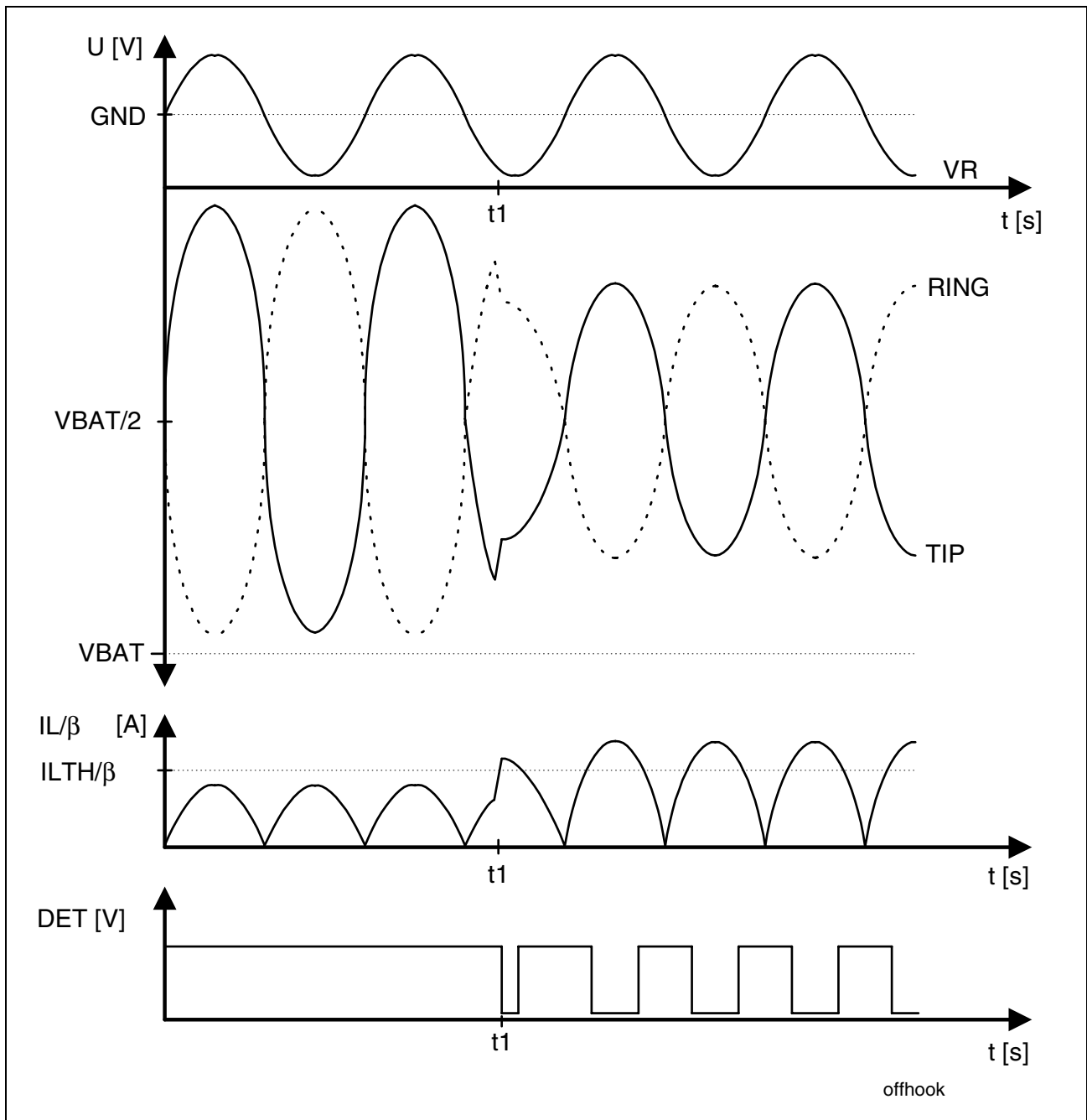
Figure 14 Off-Hook During Ringling
