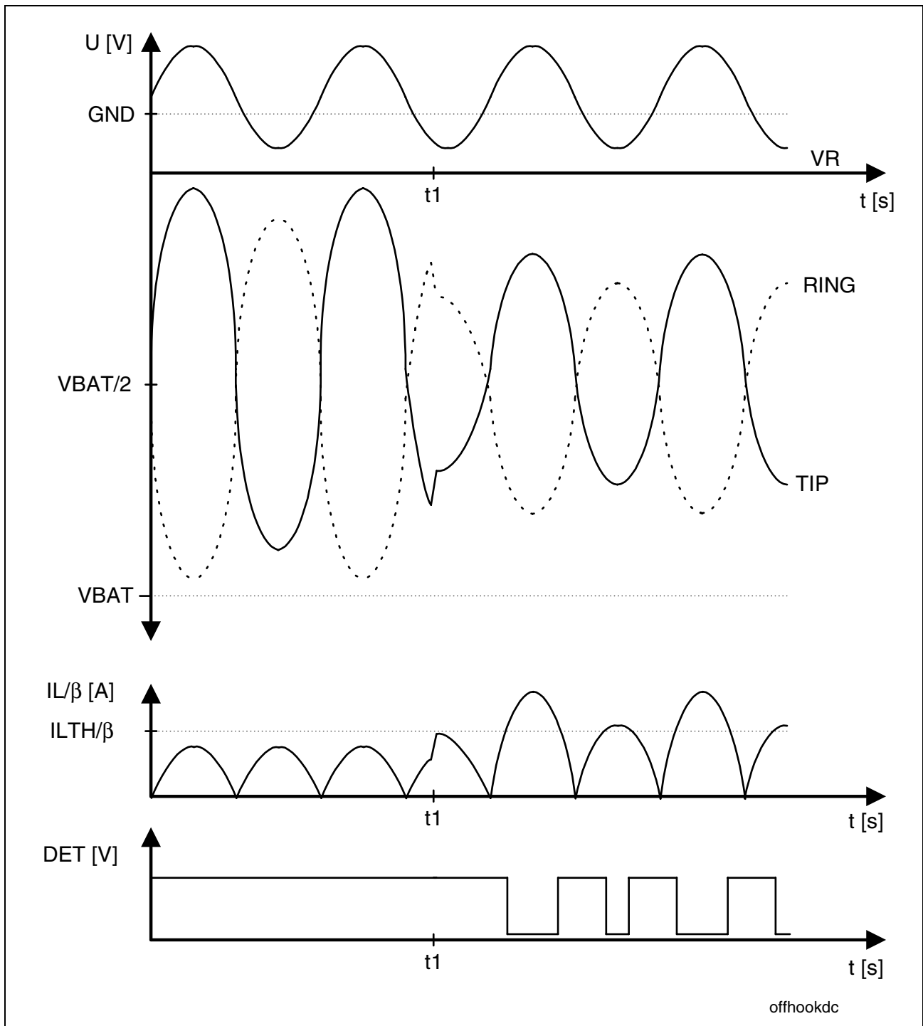
Figure 15 Off-Hook During Ringing with an Applied DC Offset
