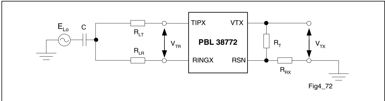
Figure 4 Longitudinal to Metallic, B_{LME} and Longitudinal to Four-Wire, B_{LFE} Balance
