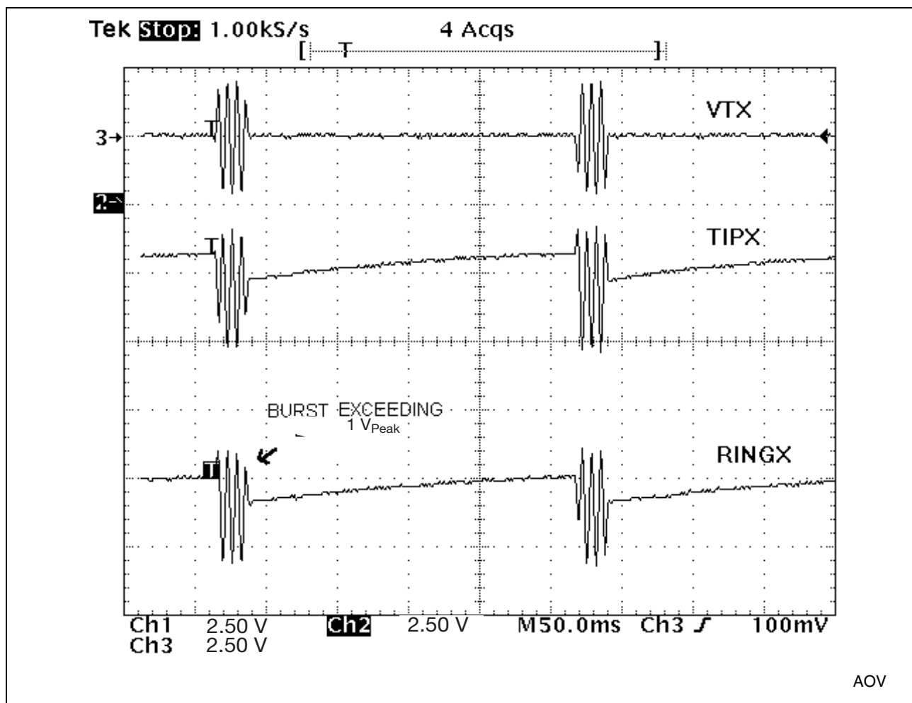
Figure 11 The AOV Function
