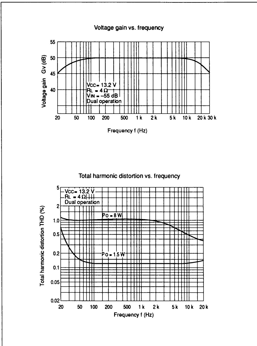
Figure 3 HA13127 Characteristic Curves (cont)
