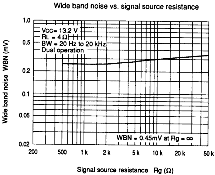
Figure 2 HA13130 Characteristic Curves (cont)
