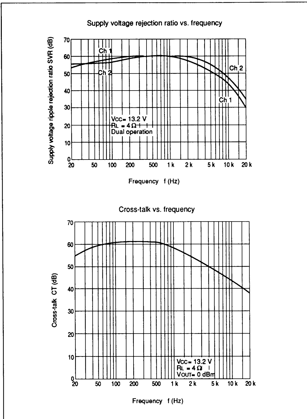
Figure 2 HA13130 Characteristic Curves (cont)
