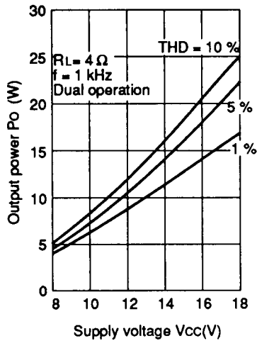
Output power vs. supply voltage (1)
