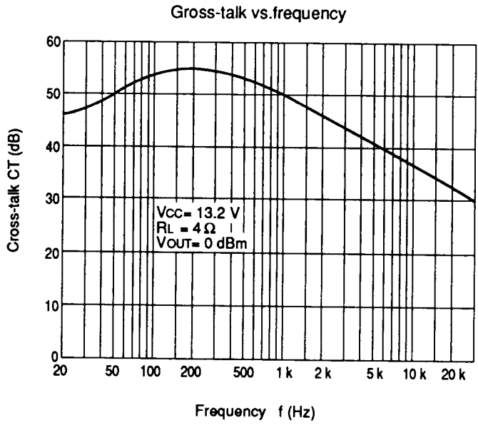
Figure 3 HA13127 Characteristic Curves (cont)
