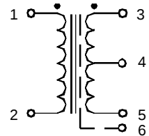
Schematic S
