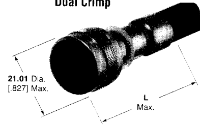
Hex Dual Crimp
