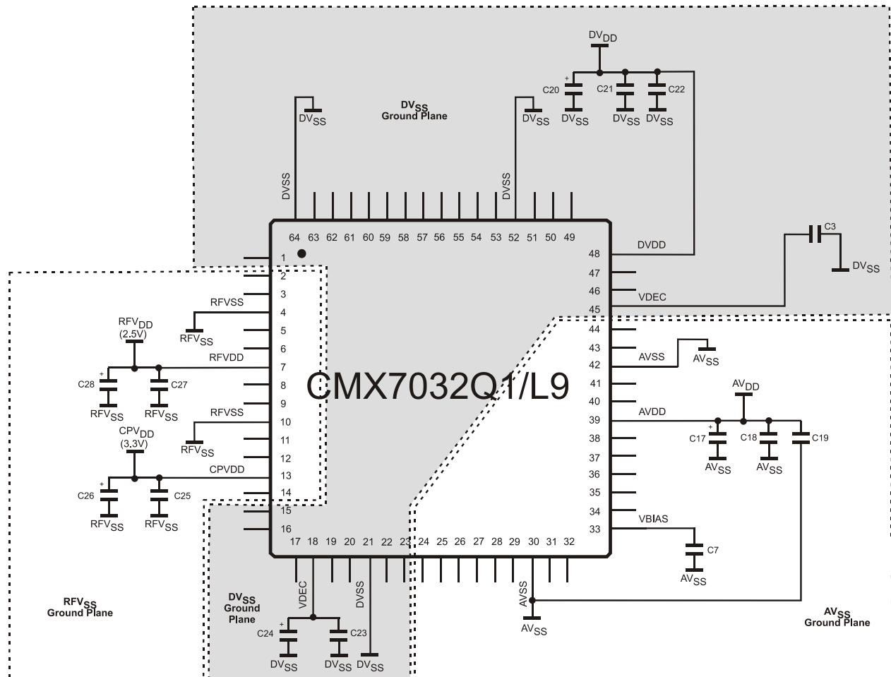
Figure 4 CMX7032 Power Supply Connections and De-coupling Component Values as per Table 2.
