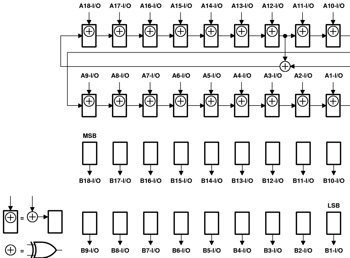
Figure 12. 18-Bit PSA/COUNT Configuration ( \overline{OEAB} = 0, \overline{OEBA} = 1 )
