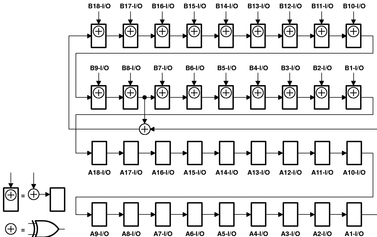
Figure 9. 36-Bit PSA Configuration ( \overline{OEAB} = 1, \overline{OEBA} = 0 )
