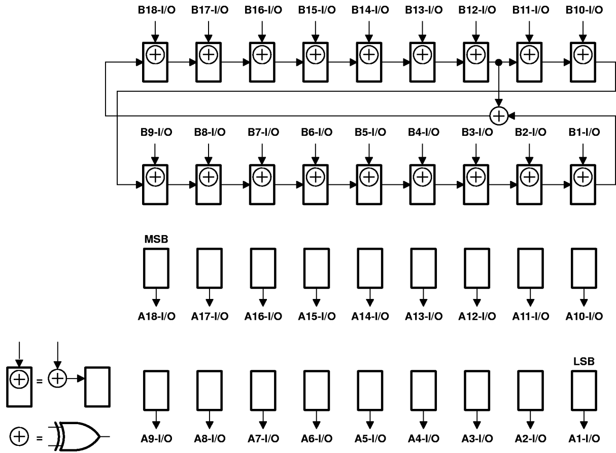
Figure 13. 18-Bit PSA/COUNT Configuration ( \overline{OEAB} = 1 , \overline{OEBA} = 0 )
