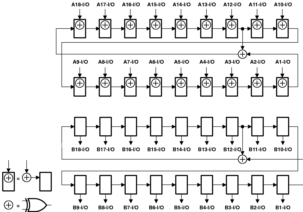
Figure 10. 18-Bit PSA/PRPG Configuration ( \overline{OEAB} = 0, \overline{OEBA} = 1 )
