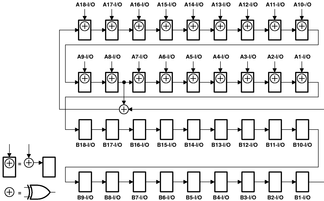
Figure 8. 36-Bit PSA Configuration ( \overline{OEAB} = 0, \overline{OEBA} = 1 )
