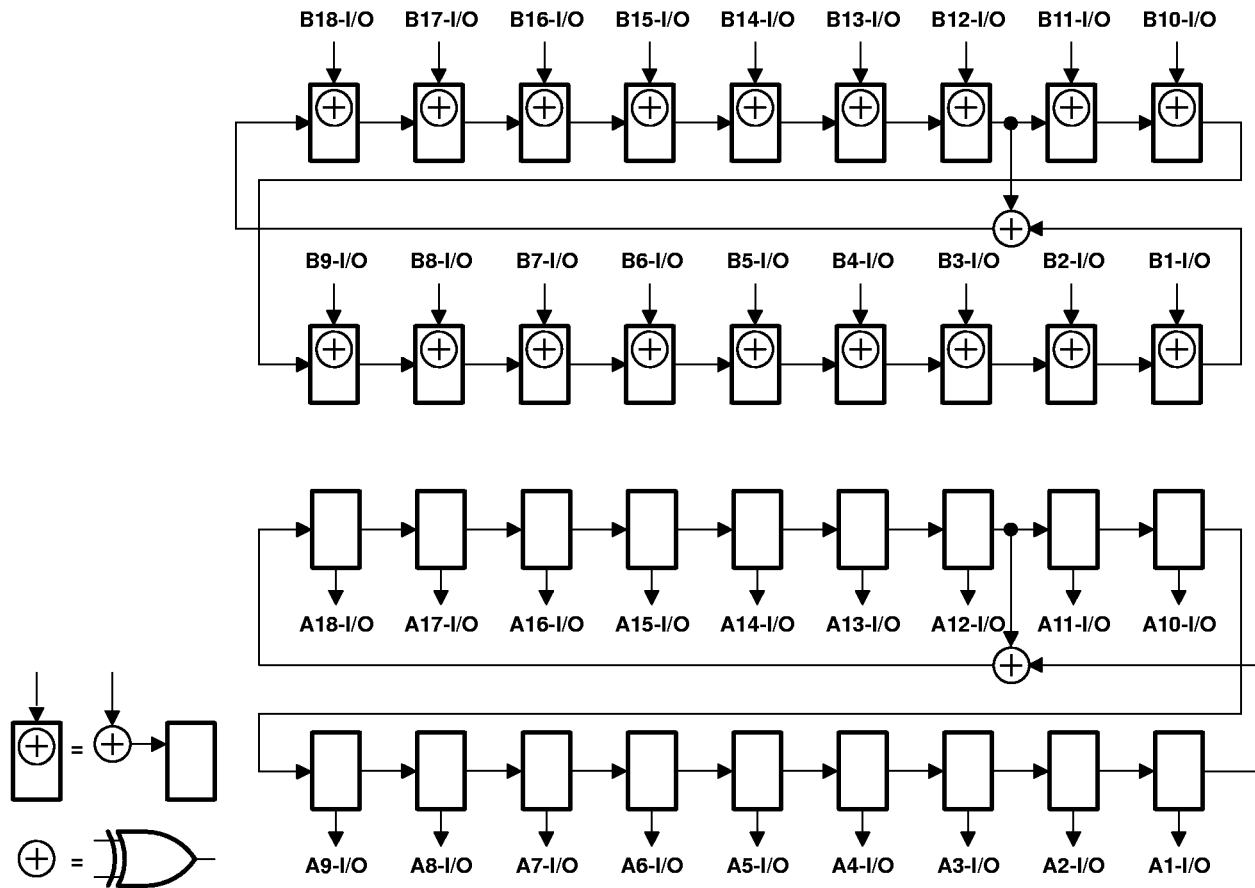
Figure 11. 18-Bit PSA/PRPG Configuration ( \overline{OEAB} = 1 , \overline{OEBA} = 0 )
