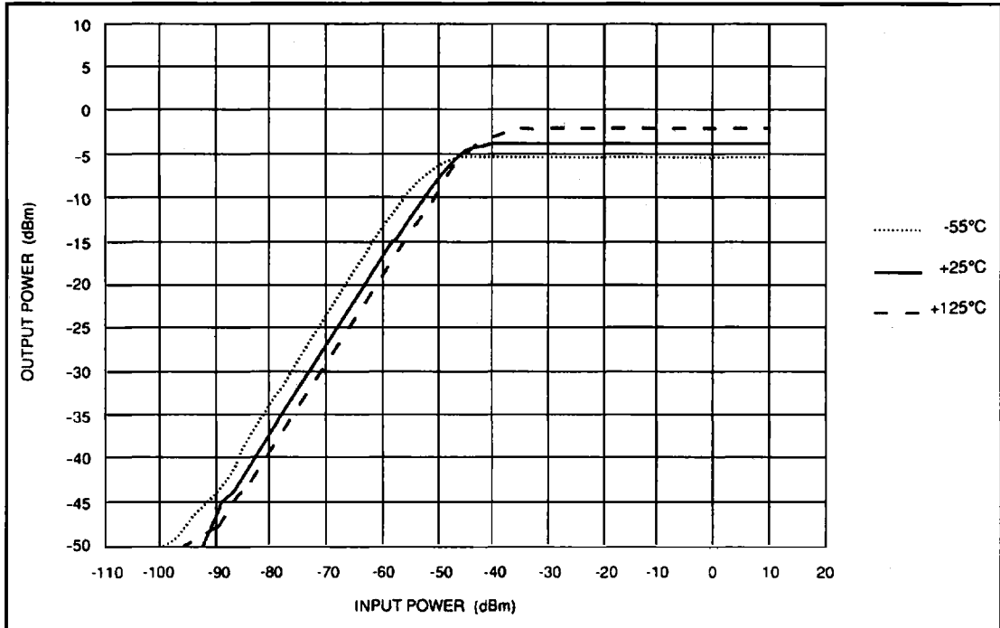
Fig.18 IF limiting characteristic at 500MHz across temperature
