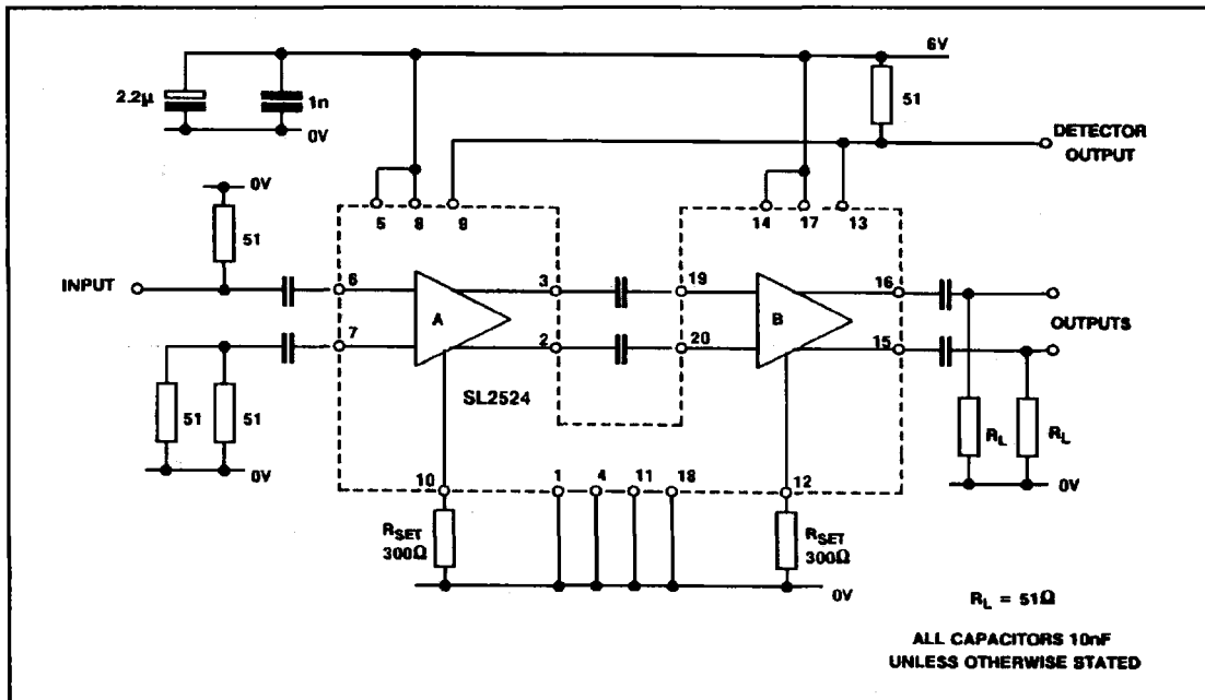
Fig.4 Test circuit
