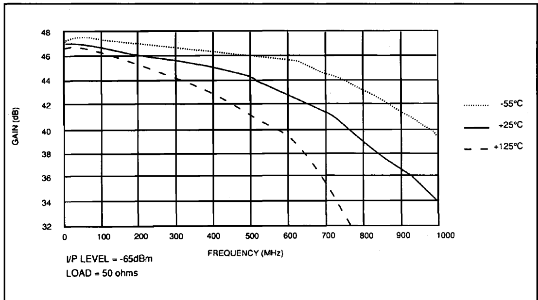
Fig.19 Small signal gain vs frequency across temperature
