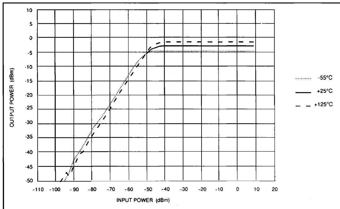
Fig. 17 IF limiting characteristic at 60MHz across temperature
