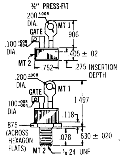
3/4" STUD-MOUNT
