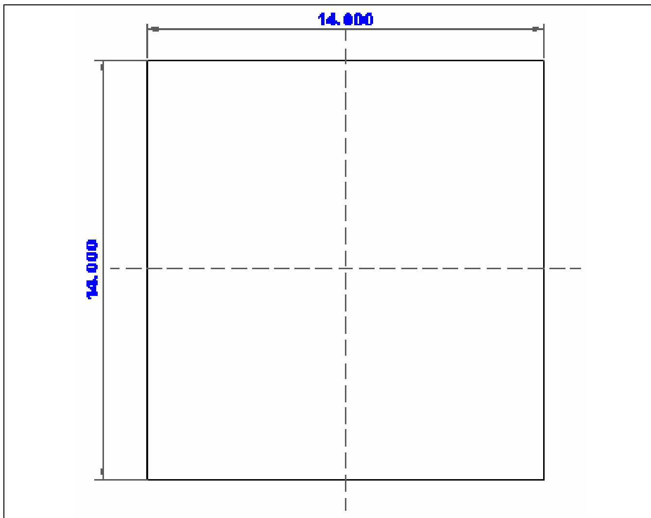
Figure 1-1. 332-FBGA SC32442X Package Dimension (Top View )
