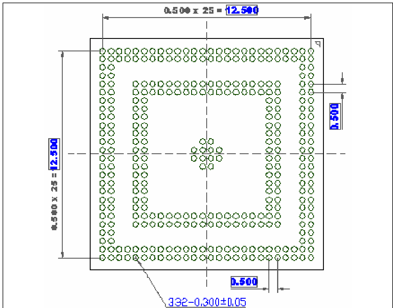
Figure 1-2. 332-FBGA SC32442X Package Dimension (Bottom View )
