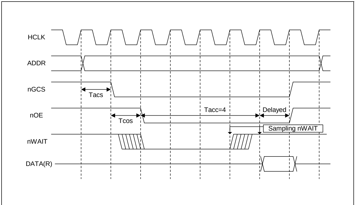
Figure 5-2. SC32442A External nWAIT Timing Diagram ( T_{acc}=4 )
