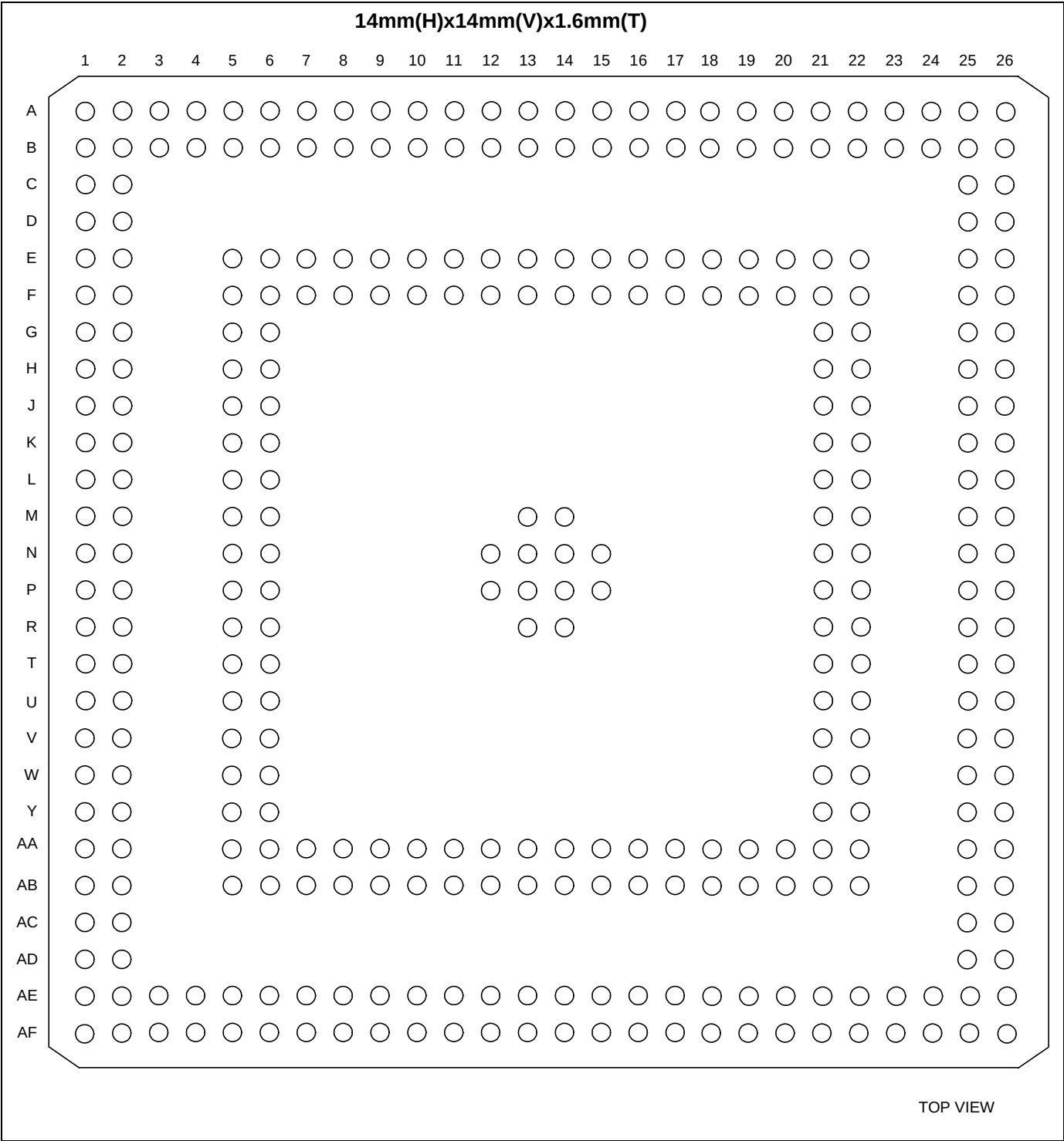
Figure 1-2. SC32442X Pin Assignments (332-FBGA)
