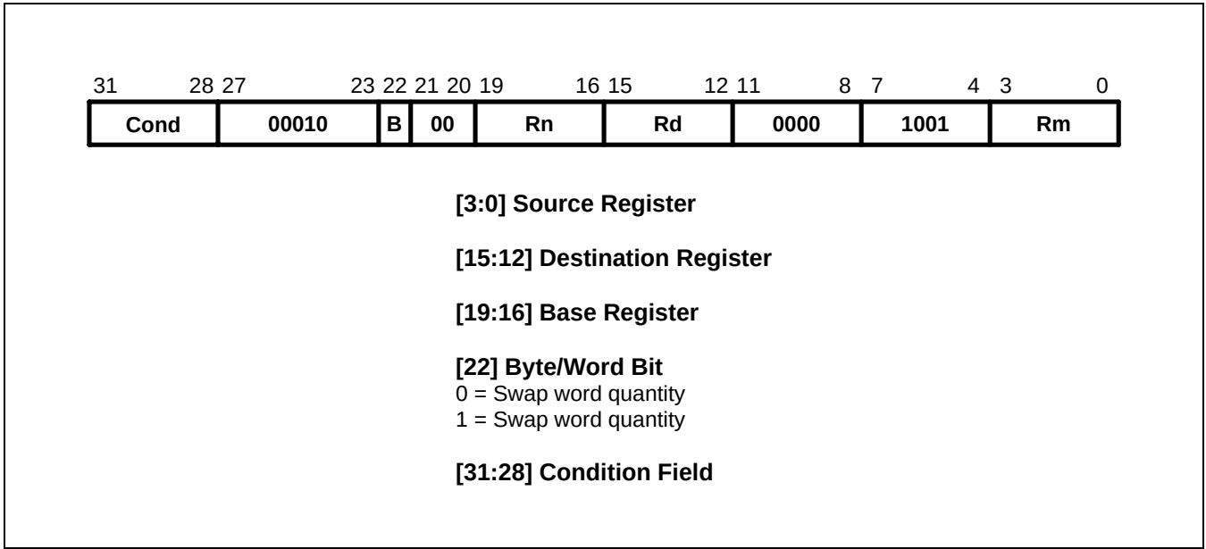
Figure 3-23. Swap Instruction
