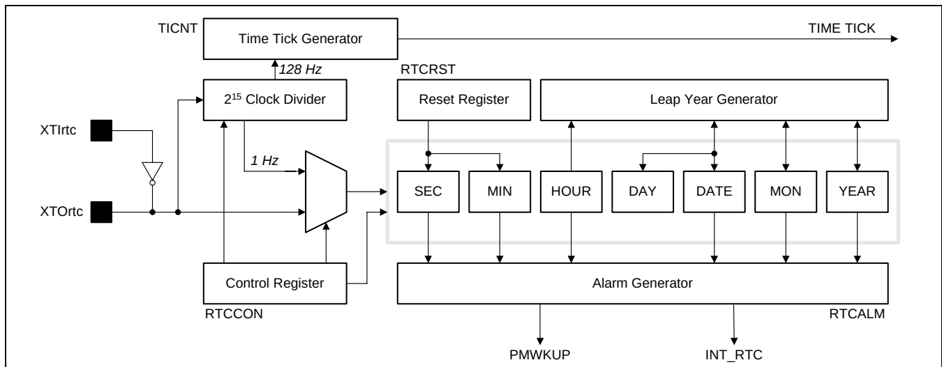
Figure 17-1. Real Time Clock Block Diagram
