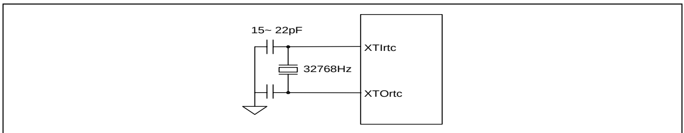
Figure 17-2. Main Oscillator Circuit Example
