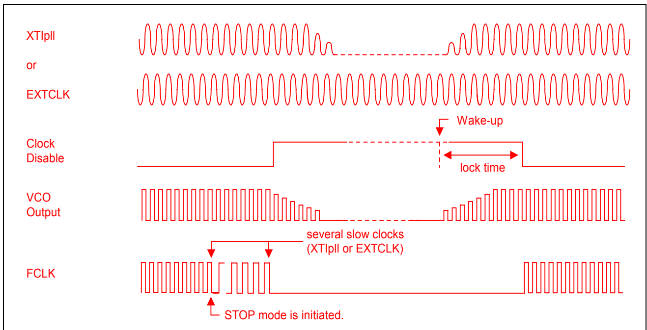
Figure7-12. Entering STOP Mode and Exiting STOP mode (Wake-up)
