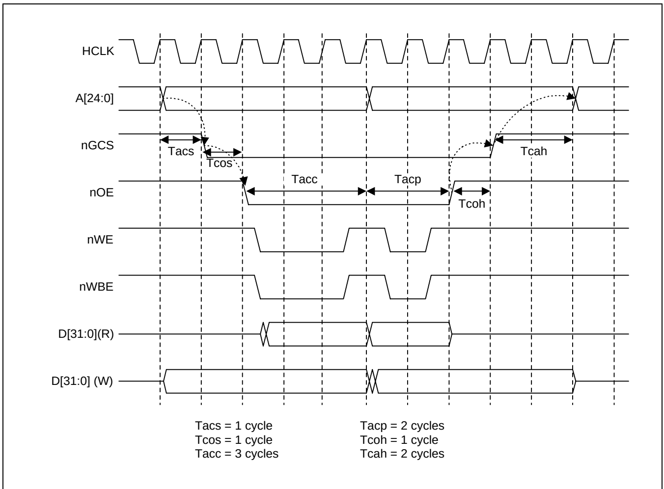
Figure 5-12. SC32442A nGCS Timing Diagram
