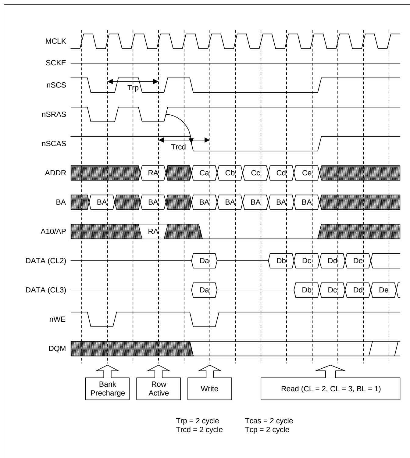
Figure 5-13. SC32442A SDRAM Timing Diagram
