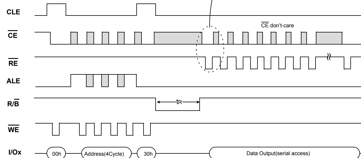
Figure 5. Read Operation with \overline{CE} don't-care.
