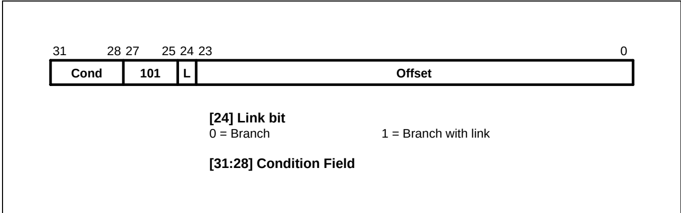
Figure 3-3. Branch Instructions
