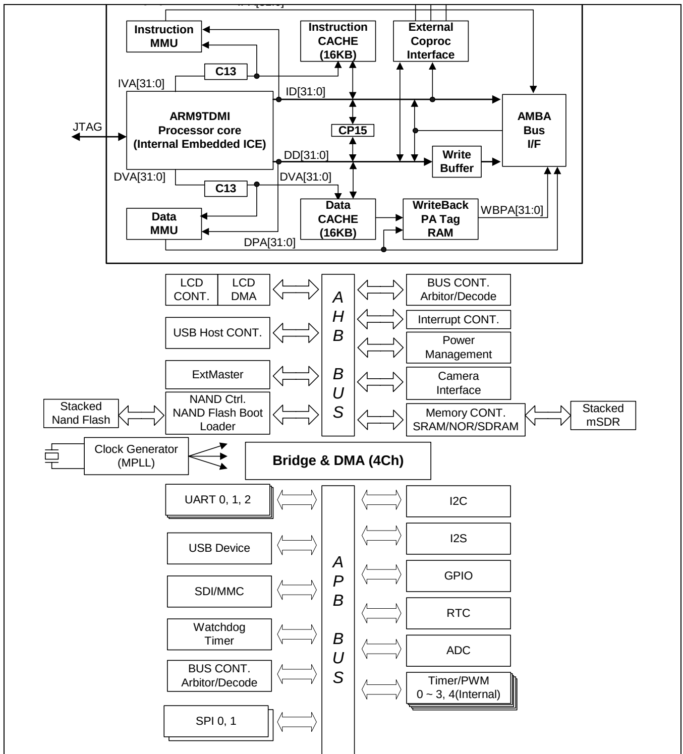
Figure 1-1. SC32442A Block Diagram
