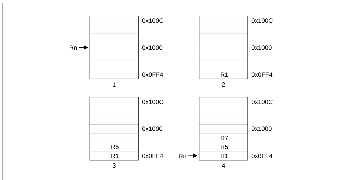
Figure 3-22. Pre-Decrement Addressing
