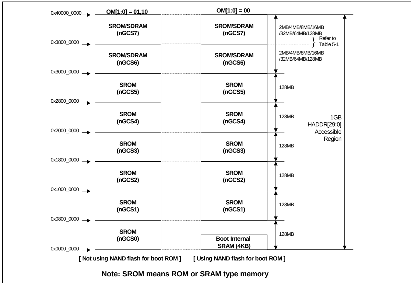
Figure 5-1. SC32442A Memory Map after Reset
