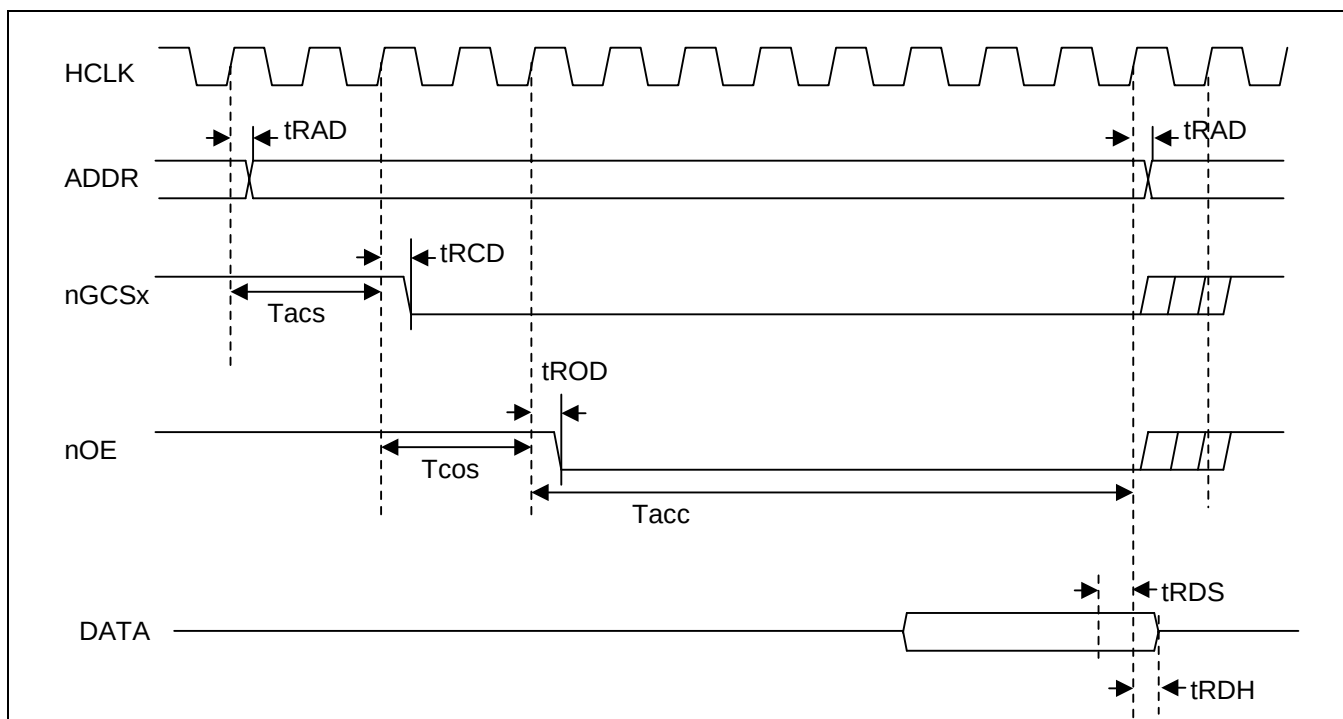
Figure 25-17 Masked-ROM Single READ Timing Diagram ( T_{acs}=2 , T_{cos}=2 , T_{acc}=8 , PMC=01/10/11 )
