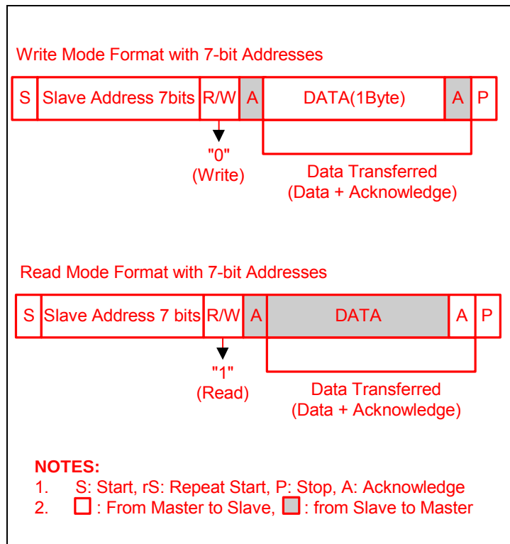
Figure 13-3. IIC-Bus Interface Data Format
