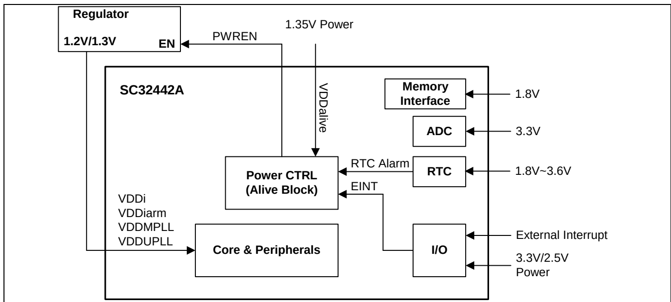
Figure 7-13. SLEEP Mode
