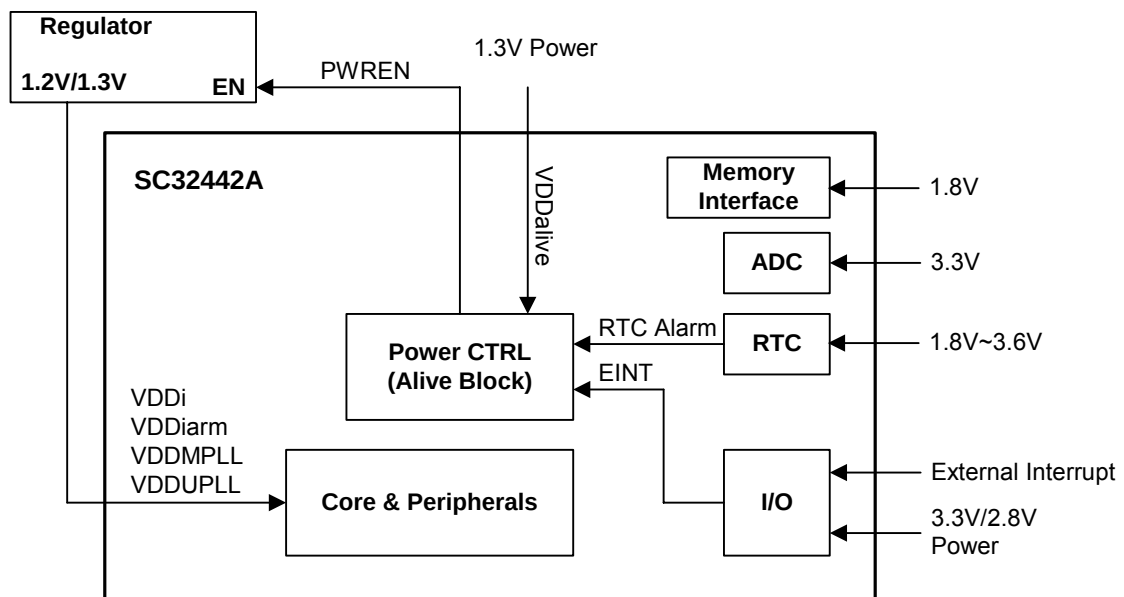
Figure 7-13. SLEEP Mode
