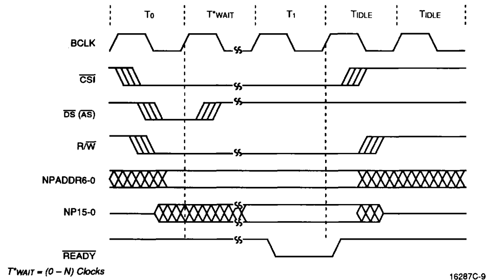
Figure 3. NP-Bus Synchronous MDRU/MDRL Read/Write Cycles
