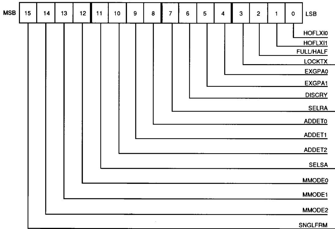
Figure 19. Mode Register 1 (MDREG1)
