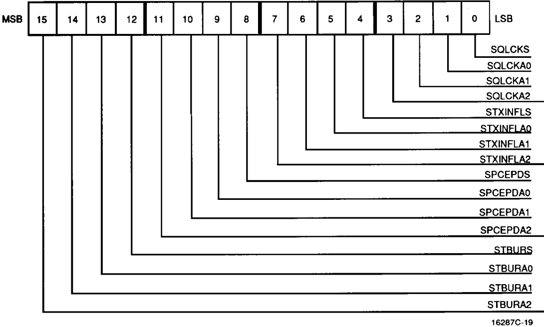
Figure 12. Status Register 1 – Lower 16 Bits (ST1L)
