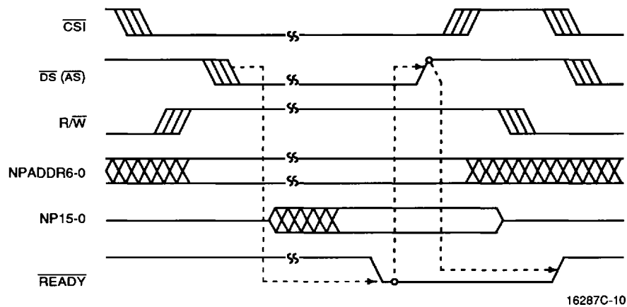
NP-Bus Asynchronous Read Cycle
