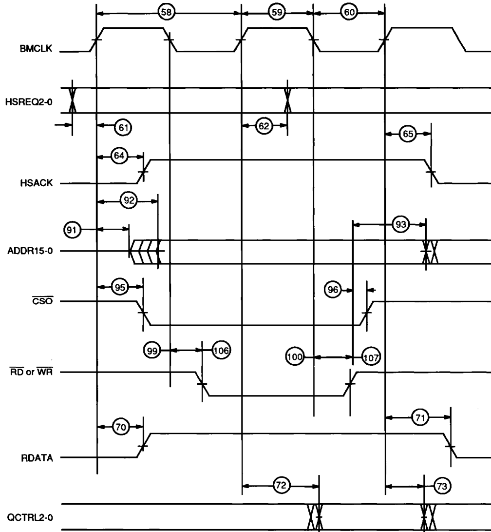
Figure 41. Host Interface Signal Timings
