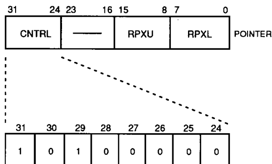
Figure 16. Format of Pointer (Nontag Mode)
