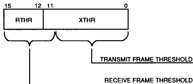
Figure 23. Frame Threshold Register
