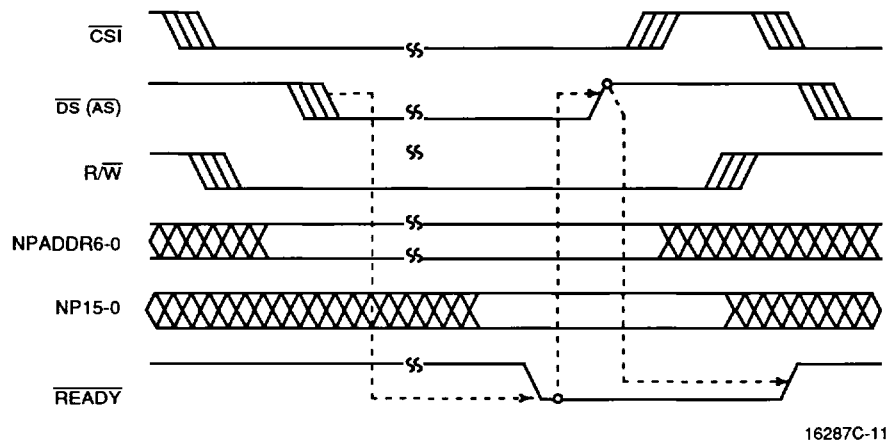
NP-Bus Asynchronous Write Cycle
