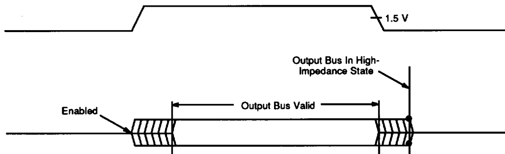
Figure 47. Output Waveform Test Points
