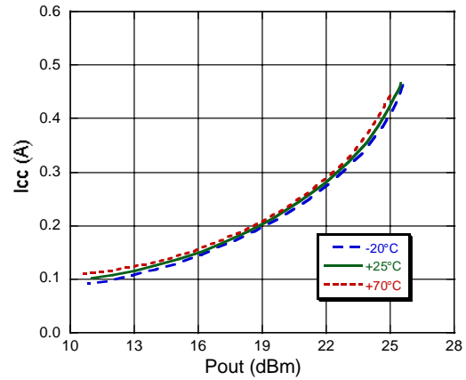
I_{CC} vs. P_{OUT} and Temp @ 2.4 V, 2450 MHz
