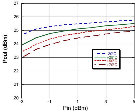
P_{OUT} vs. P_{IN} and Temp @ 2.4 V, 2450 MHz
