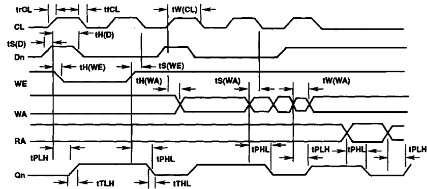
FIGURE 10. TIMING DIAGRAM
