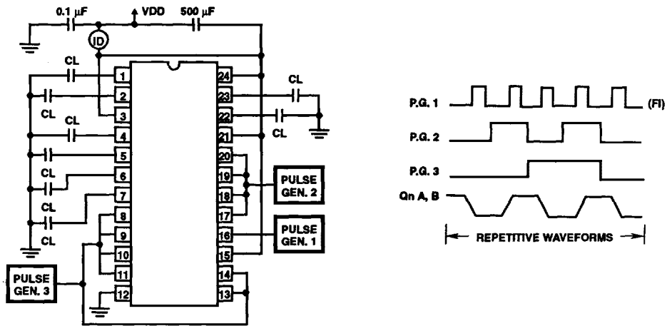
FIGURE 11. POWER-DISSIPATION TEST CIRCUIT AND WAVEFORMS
