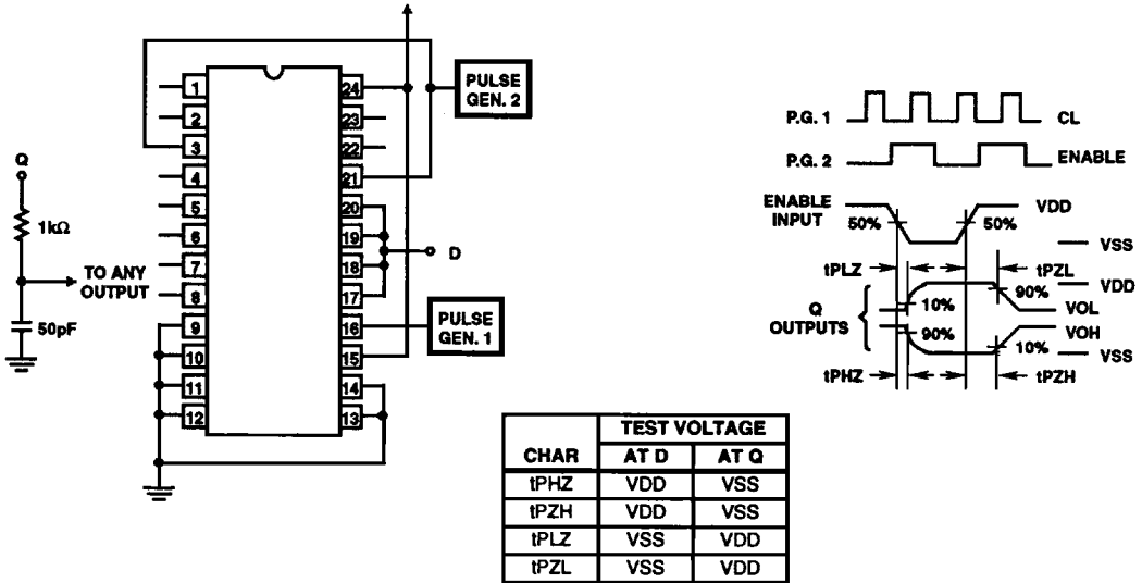
FIGURE 12. OUTPUT-ENABLE-DELAY-TIMES TEST CIRCUIT AND WAVEFORMS
