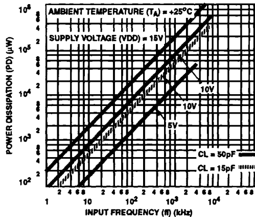
FIGURE 8. TYPICAL POWER DISSIPATION AS A FUNCTION OF INPUT FREQUENCY
