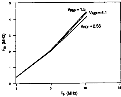
DNL VS. INPUT BANDWIDTH AS A FUNCTION OF SAMPLE RATE (DNL IS THE LARGEST ERROR APPEARING ON THE HISTOGRAM)
