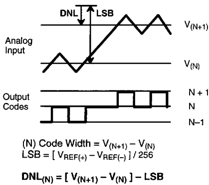
Figure 3. DNL Measurement
