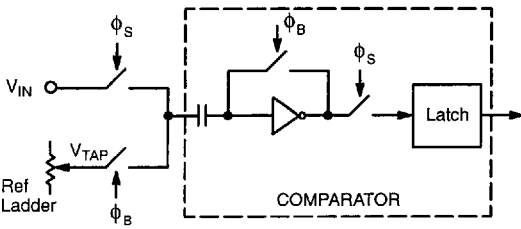
Figure 6. MP7684 Comparator
