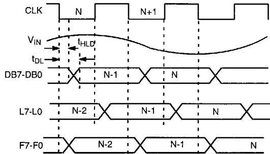
Figure 10. MP7684 Functional Equivalent Circuit and Interface Timing
