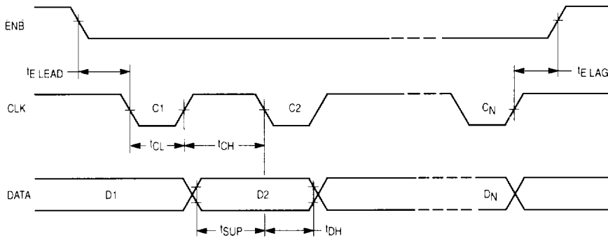
Figure 2b. Serial Input, Negative Clock
