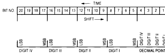
Figure 1. Input Sequence
