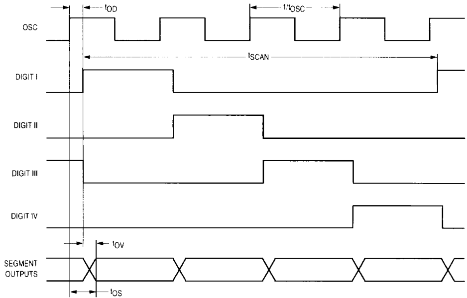
Figure 4. Scanner Waveforms
