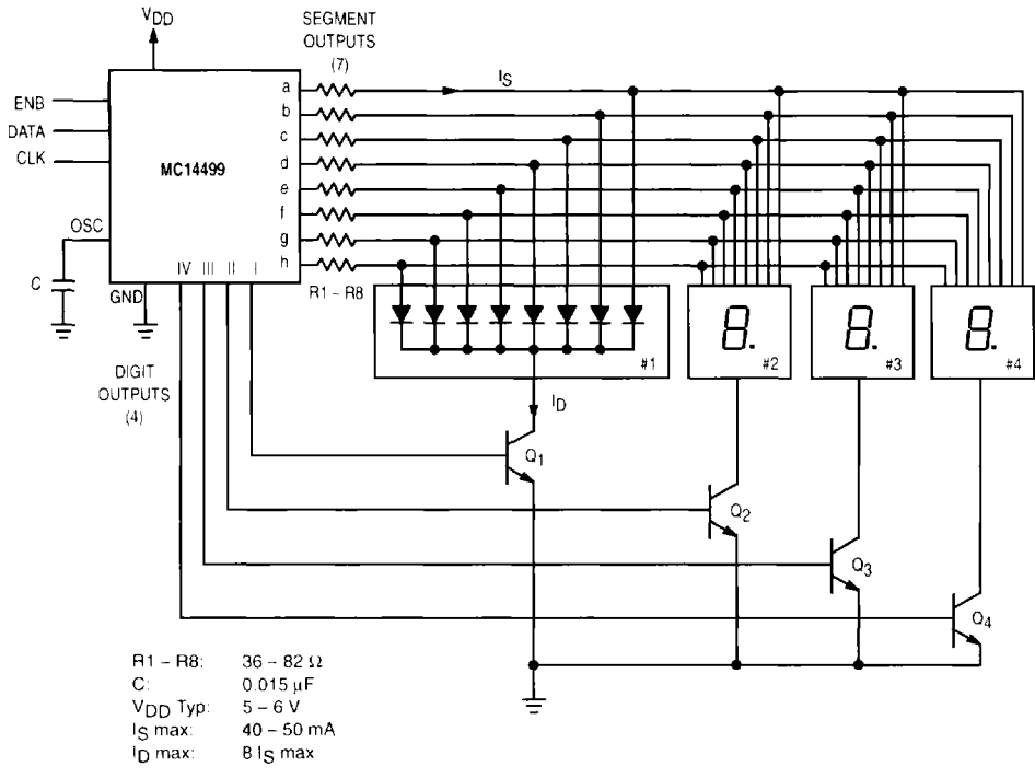
Figure 6. Application Example
