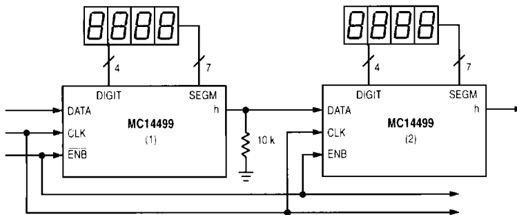
Figure 3. Cascading MC14499s
