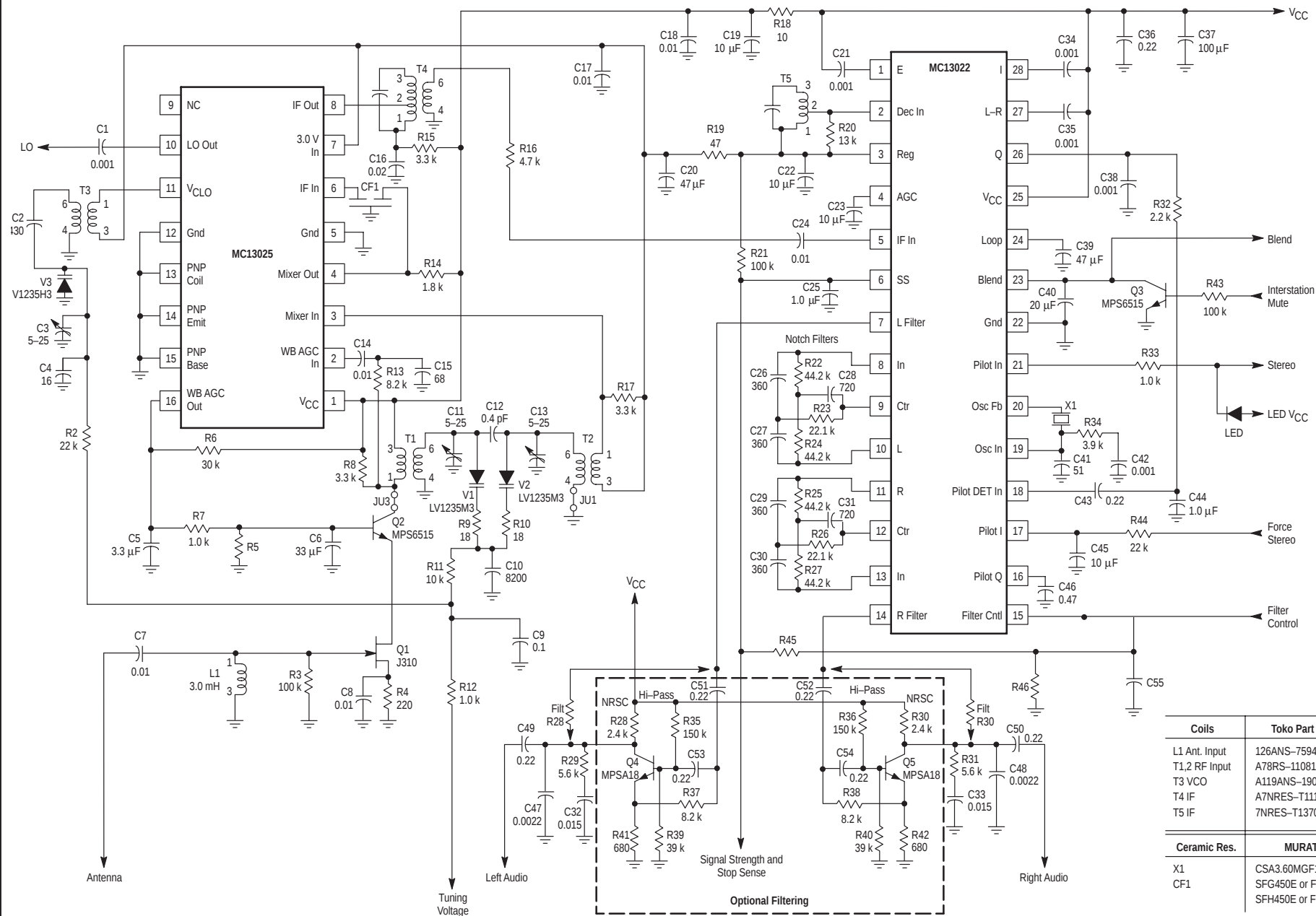
Figure 2. Cascode RF ETR Application
