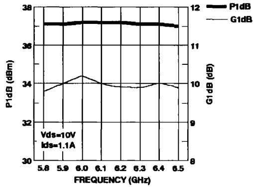
Figure 1. IM5964-4L Output Power, Gain vs. Frequency.
