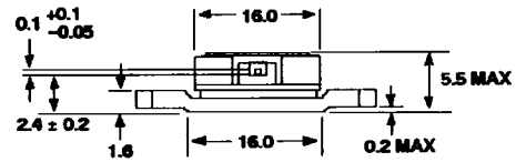
Figure 14. C24A Package Outline IM5964-16L and IM5964-32L.
