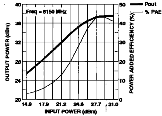
Figure 2. IM5964-4L Output Power, Power Added Efficiency vs. Input Power.
