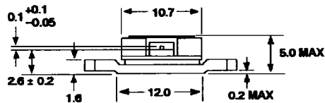
Figure 13. C21A Package Outline IM5964-4L and IM5964-8L.
