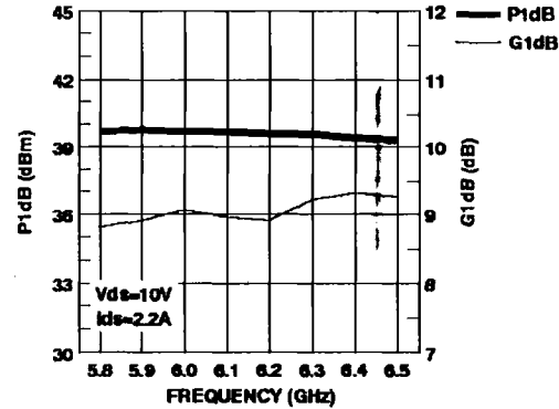
Figure 4. IM5964-8L Output Power, Gain vs. Frequency.
