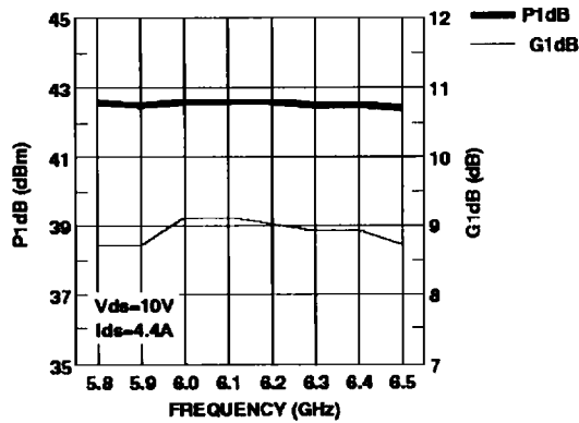
Figure 7. IM5964-16L Output Power, Gain vs. Frequency.
