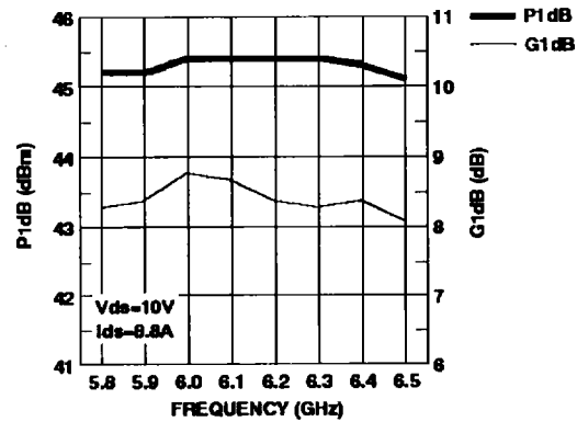
Figure 10. IM5964-32L Output Power, Gain vs. Frequency.
