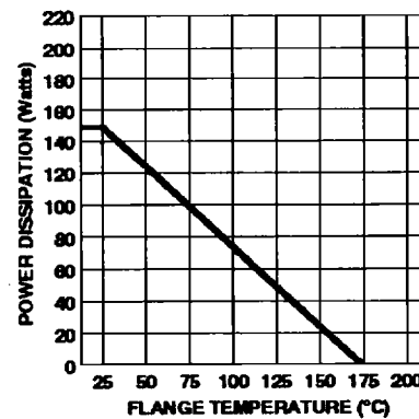
Figure 12. IM5964-32L Maximum Total Power Dissipation vs. Flange Temperature.
