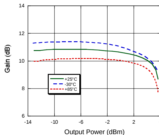
P_{1dB} @ 1635 MHz
