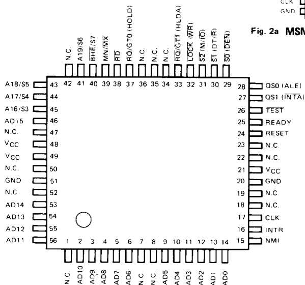
Fig. 2b MSM80C86AGS/MSM80C86A-2GS
