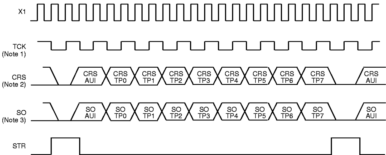
Figure 3. Minimum Mode, Non-Intelligent Repeater Example
