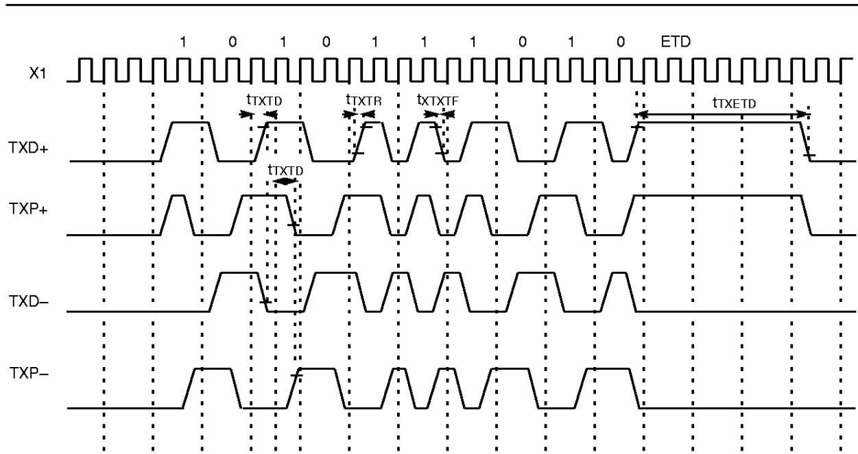
TP Ports Output Timing Diagram
