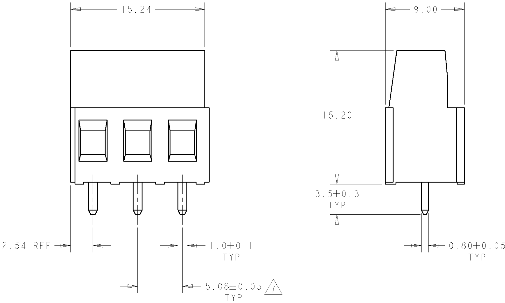
282841-3 AS SHOWN
