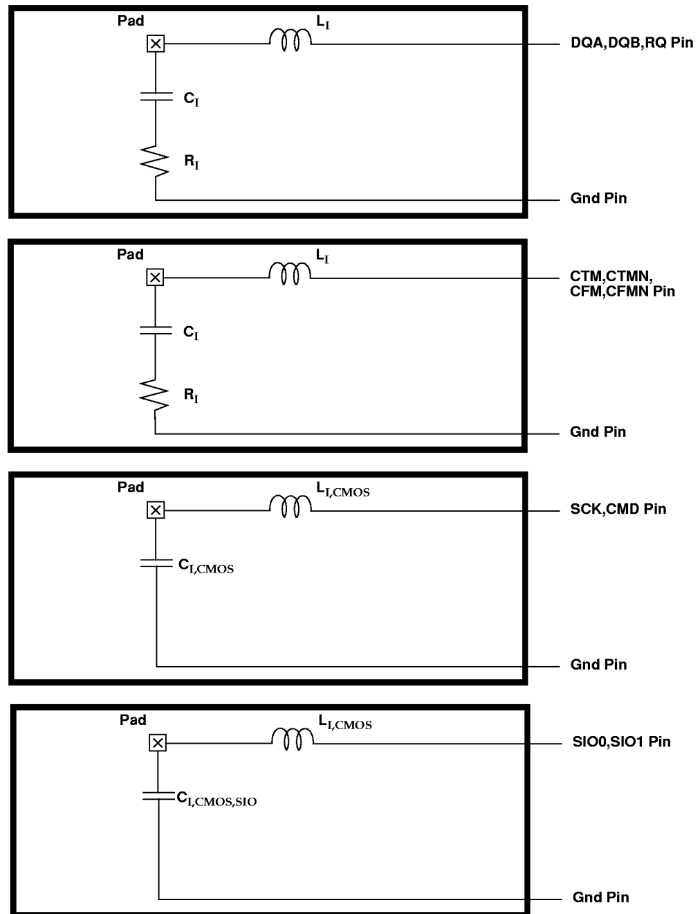
Figure 59: Equivalent Load Circuit for RSL Pins
