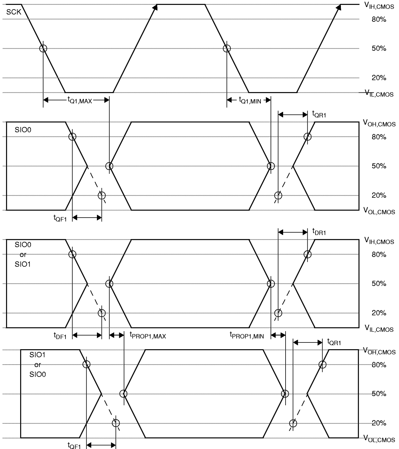
Figure 57: CMOS Timing - Data Signals for Transmit
