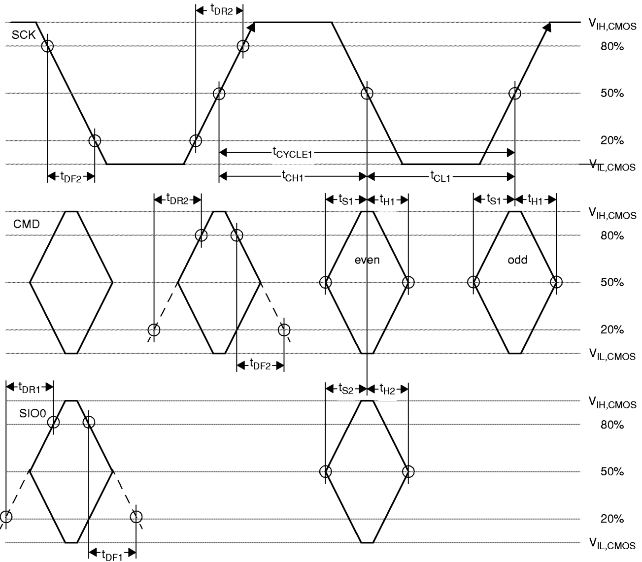
Figure 55: CMOS Timing - Data Signals for Receive
