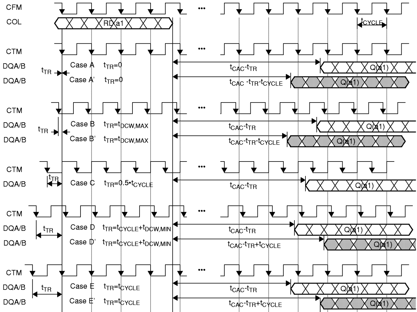
Figure 58: RSL Transmit - Crossing Read Domains
