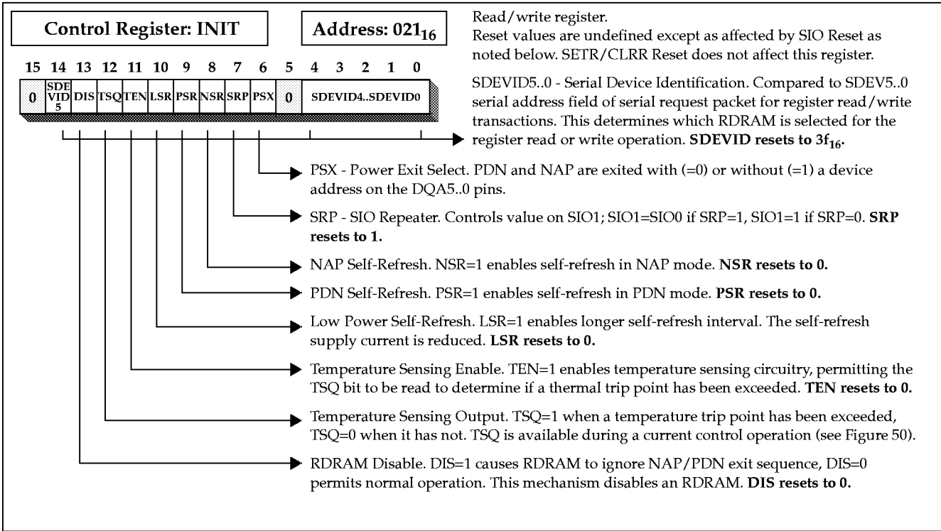
Figure 27: INIT Register
