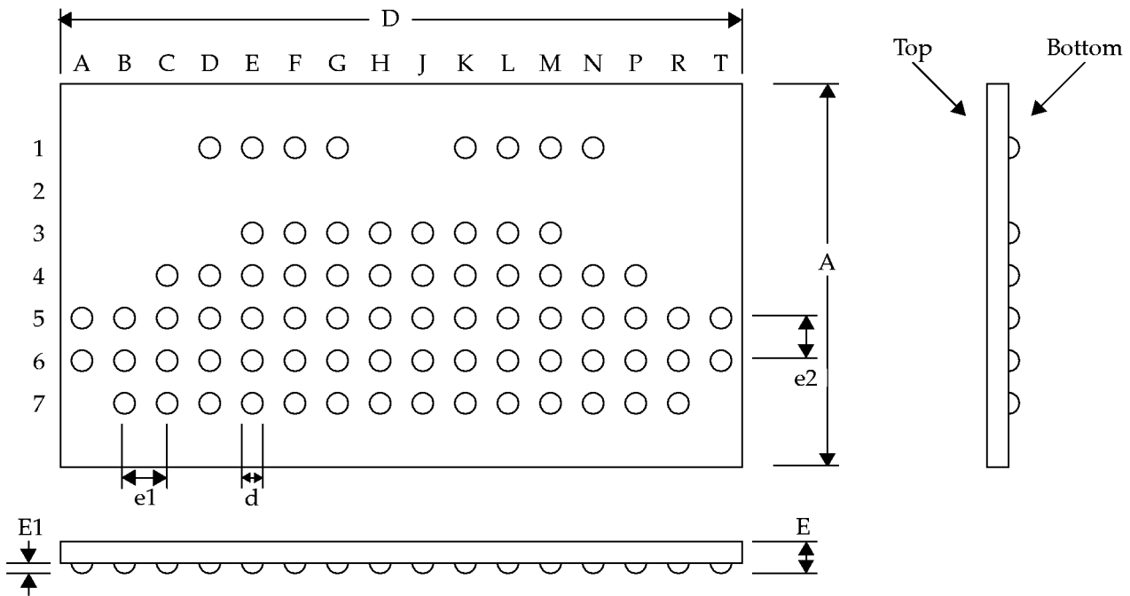
Figure 60: Edge-Bonded uBGA Package
