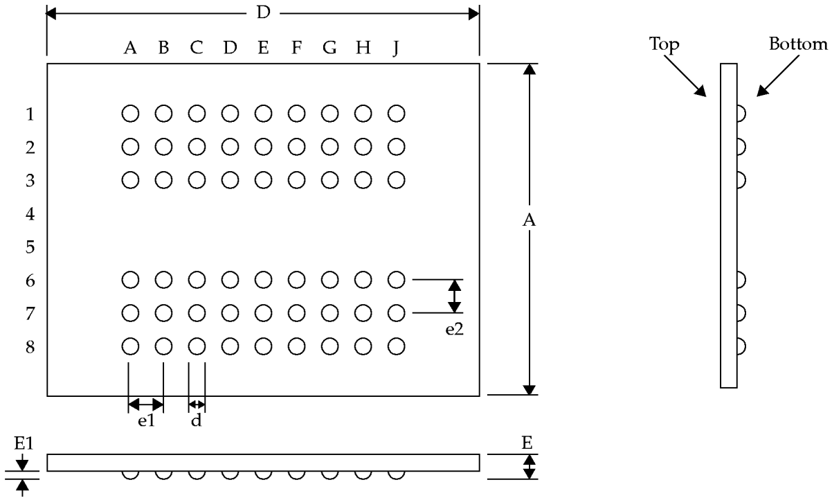
Figure 61: Center-Bonded uBGA Package
