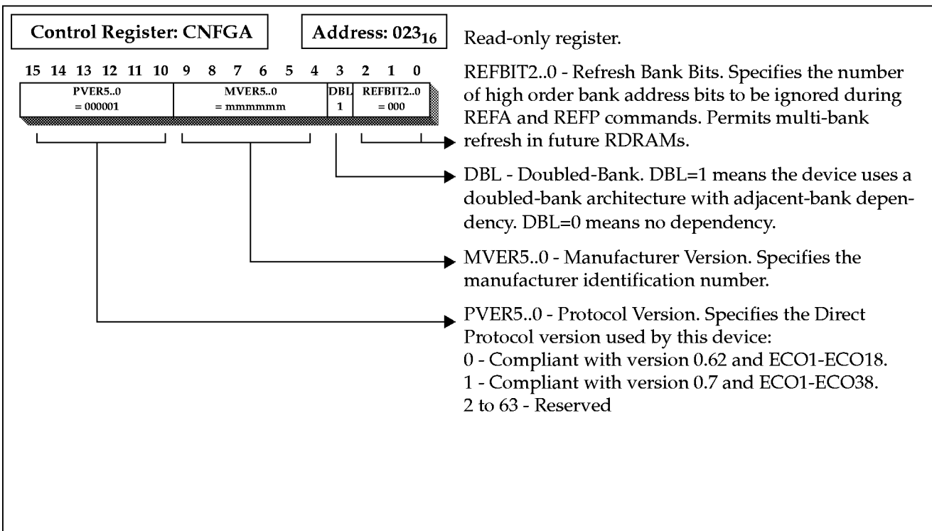
Figure 28: CNFGA Register
