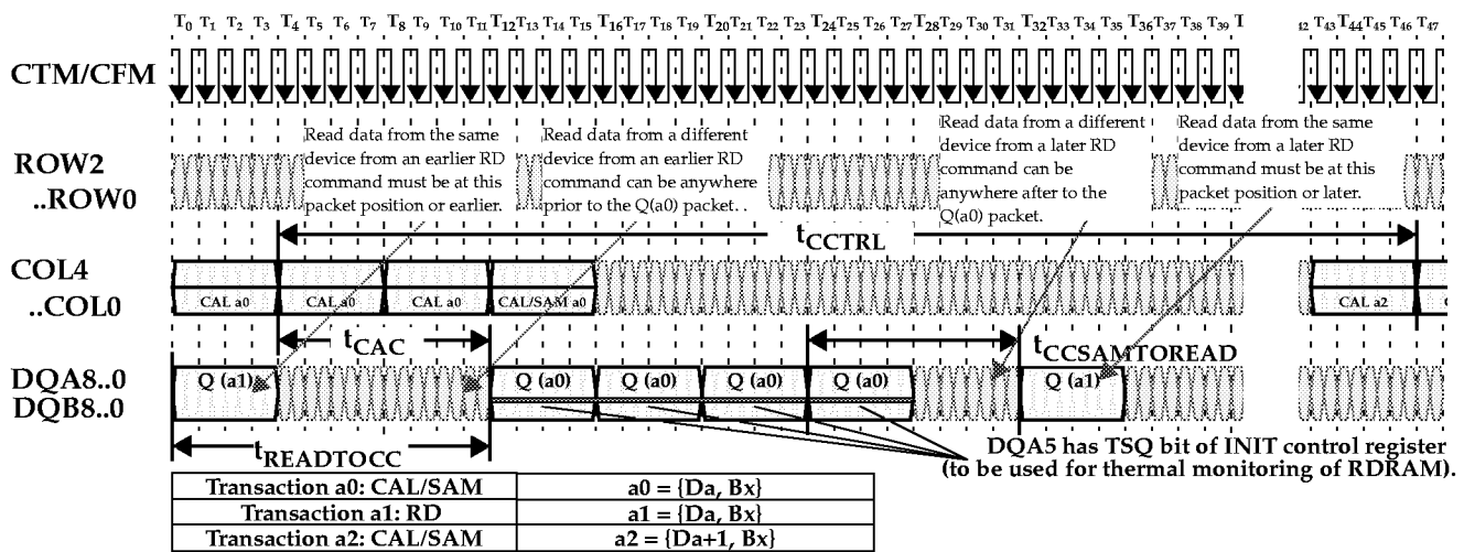
Figure 50: Current Control CAL/SAM Transaction Example
