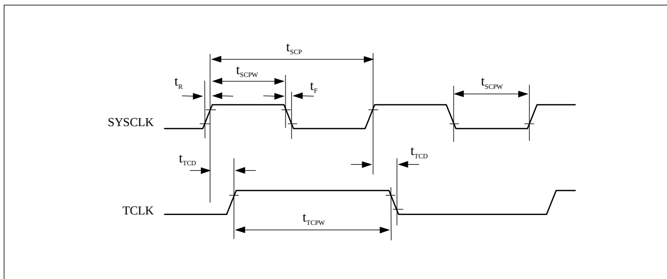
Figure 45. Clock Timing
