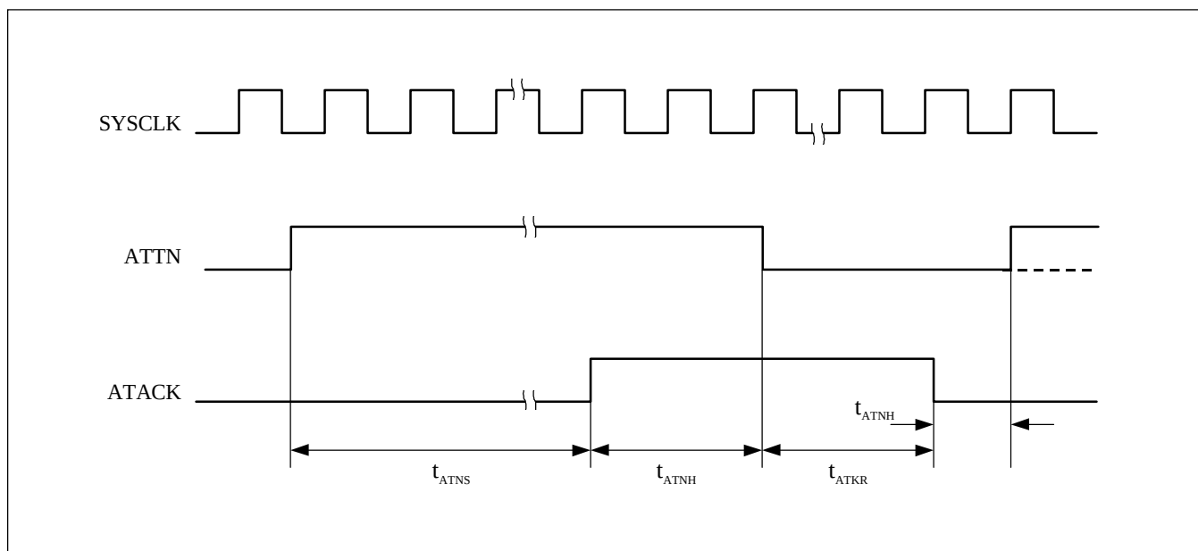
Figure 50. Channel Activation/Deactivation Timing
