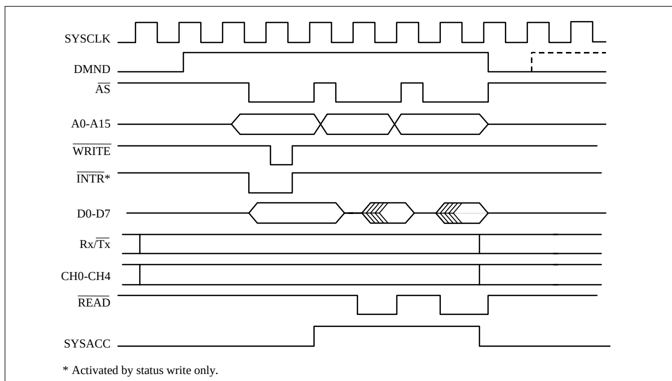
Figure 42. PT7A6632 External Memory Example Interface Waveforms - Single Write Memory Access Plus a Double Activation Read Access
