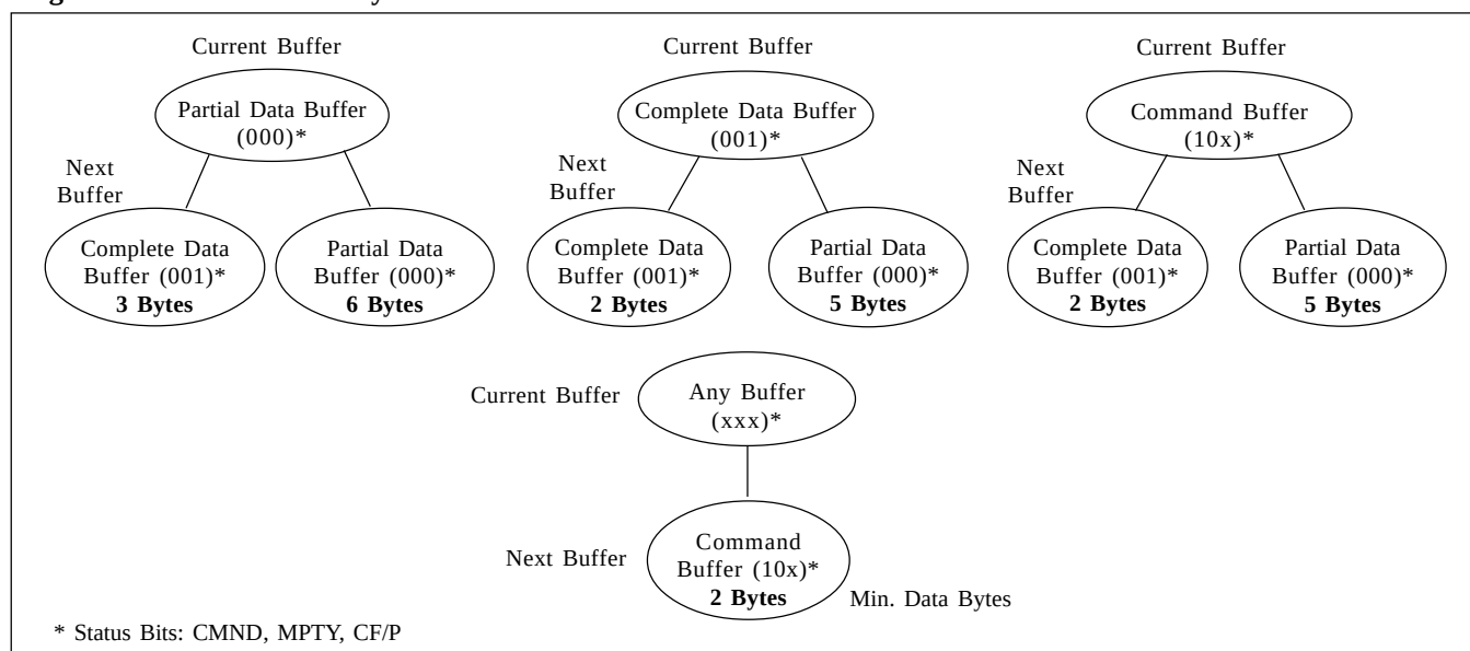
Figure 25. Minimum Data Bytes for Transmit Buffer
