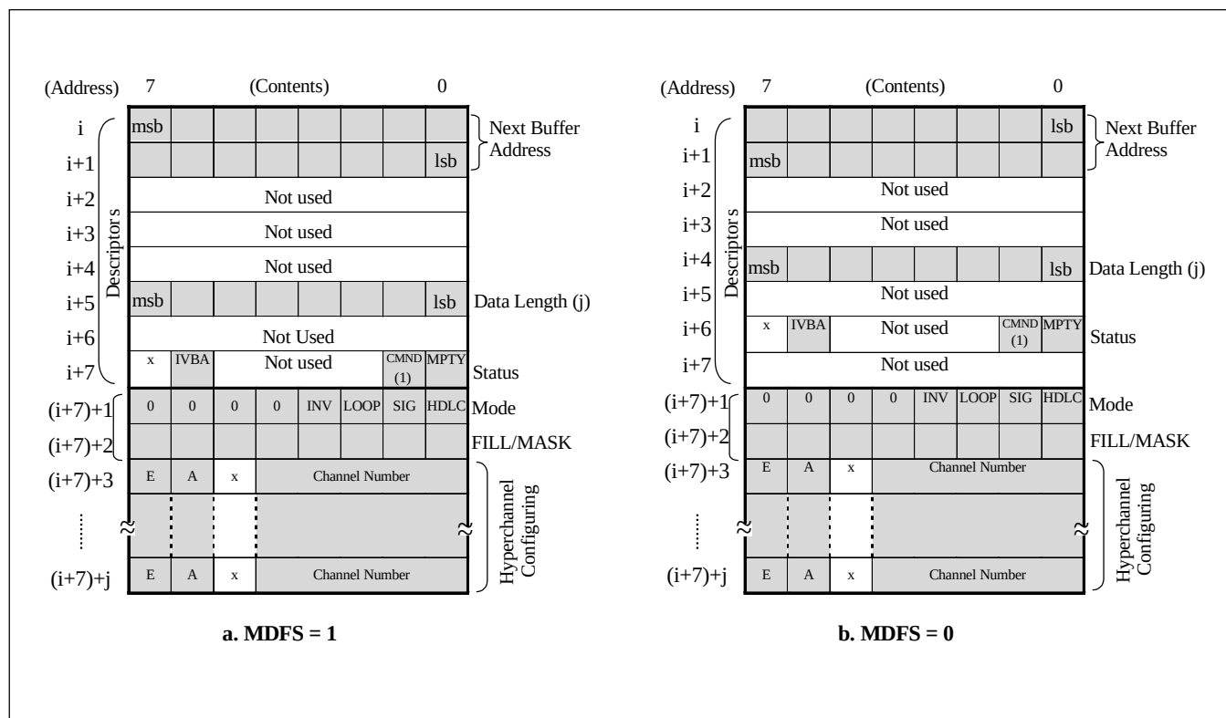
Figure 27. Receive Command Buffer
