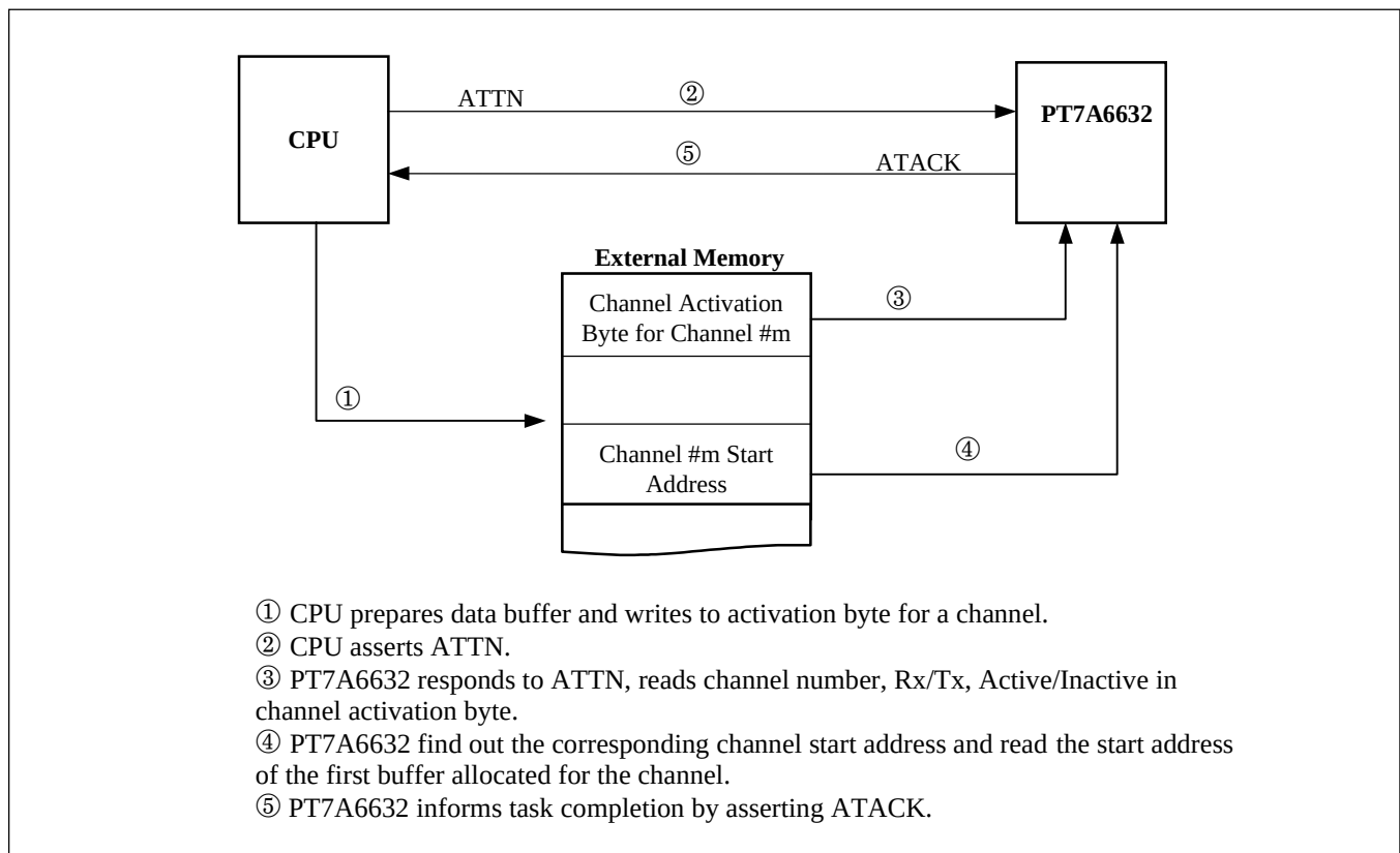
Figure 28. Channel Initialization
