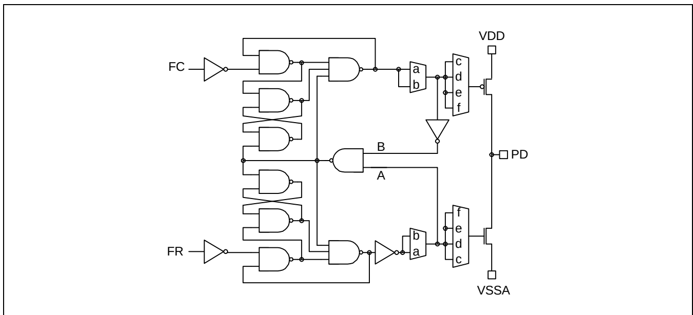
Figure 10. PFD scheme
