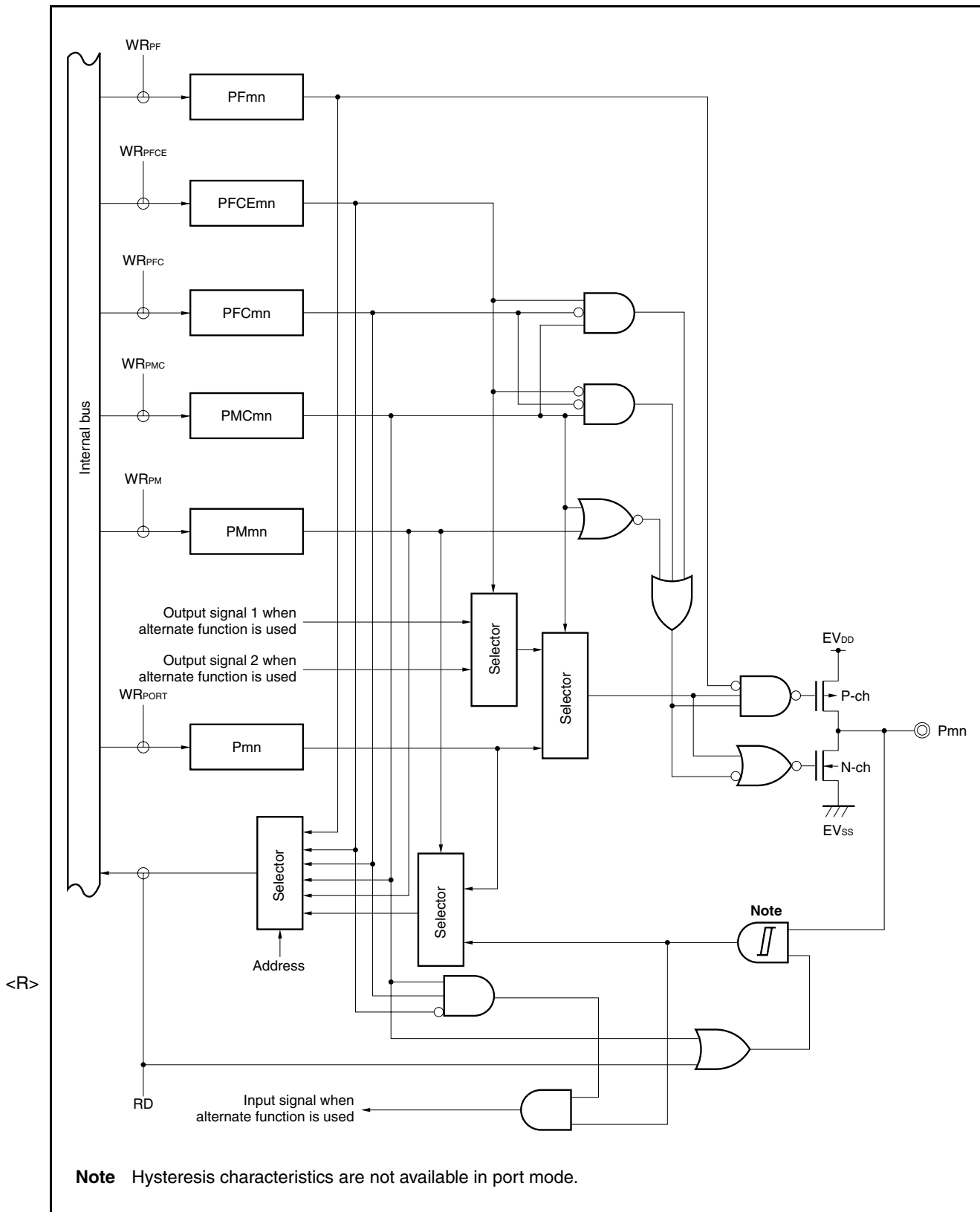
Figure 4-36. Block Diagram of Type U-12
