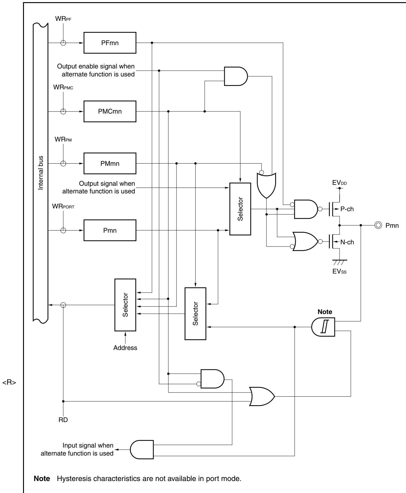
Figure 4-12. Block Diagram of Type E-3
