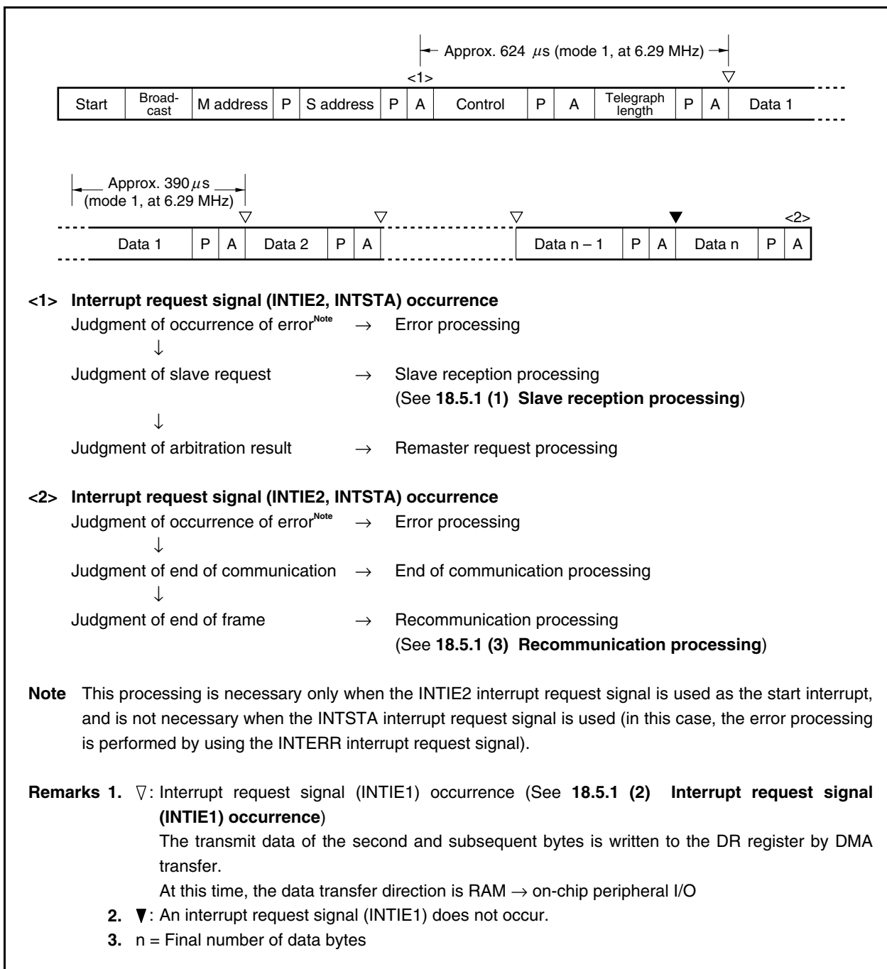
Figure 18-26. Master Transmission
