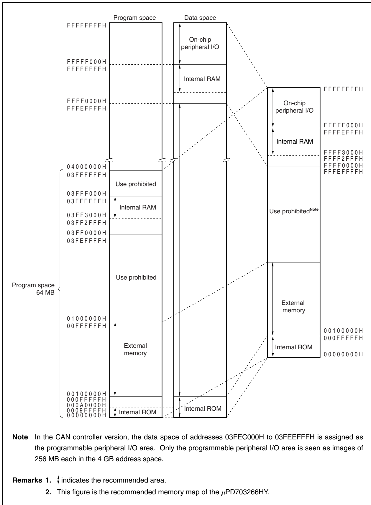
Figure 3-12. Recommended Memory Map
