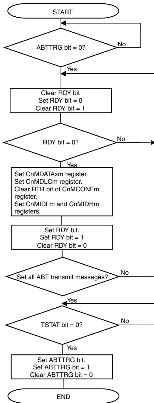
Figure 19-42. ABT Message Transmit Processing
