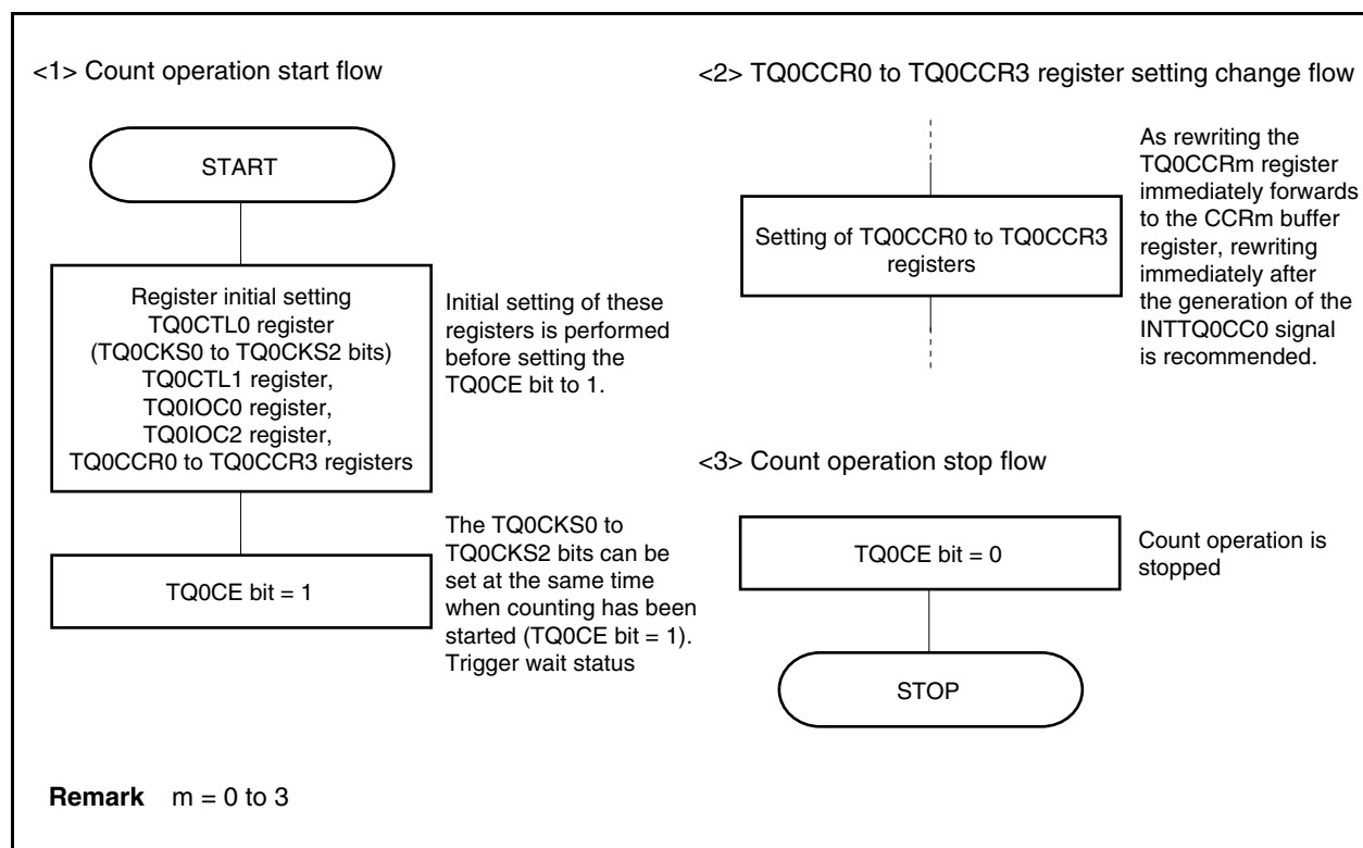
Figure 8-27. Software Processing Flow in One-Shot Pulse Output Mode (2/2)
