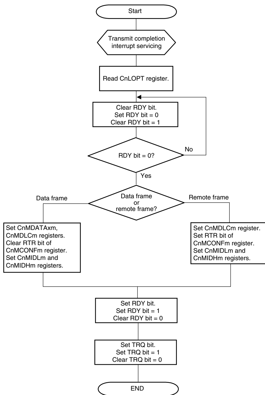
Figure 19-43. Transmission via Interrupt (Using CnLOPT Register)
