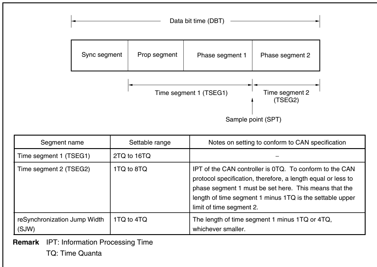
Figure 19-18. Segment Setting
