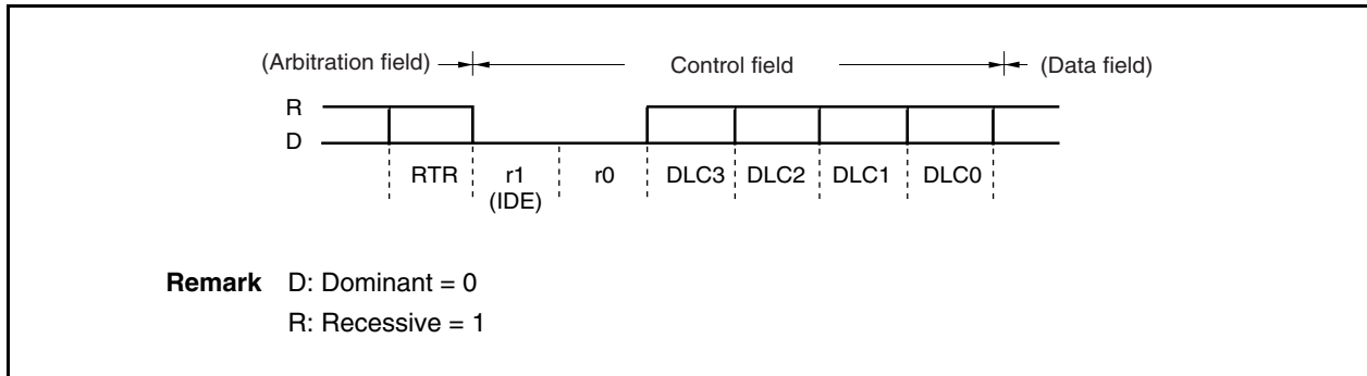
Figure 19-8. Control Field
