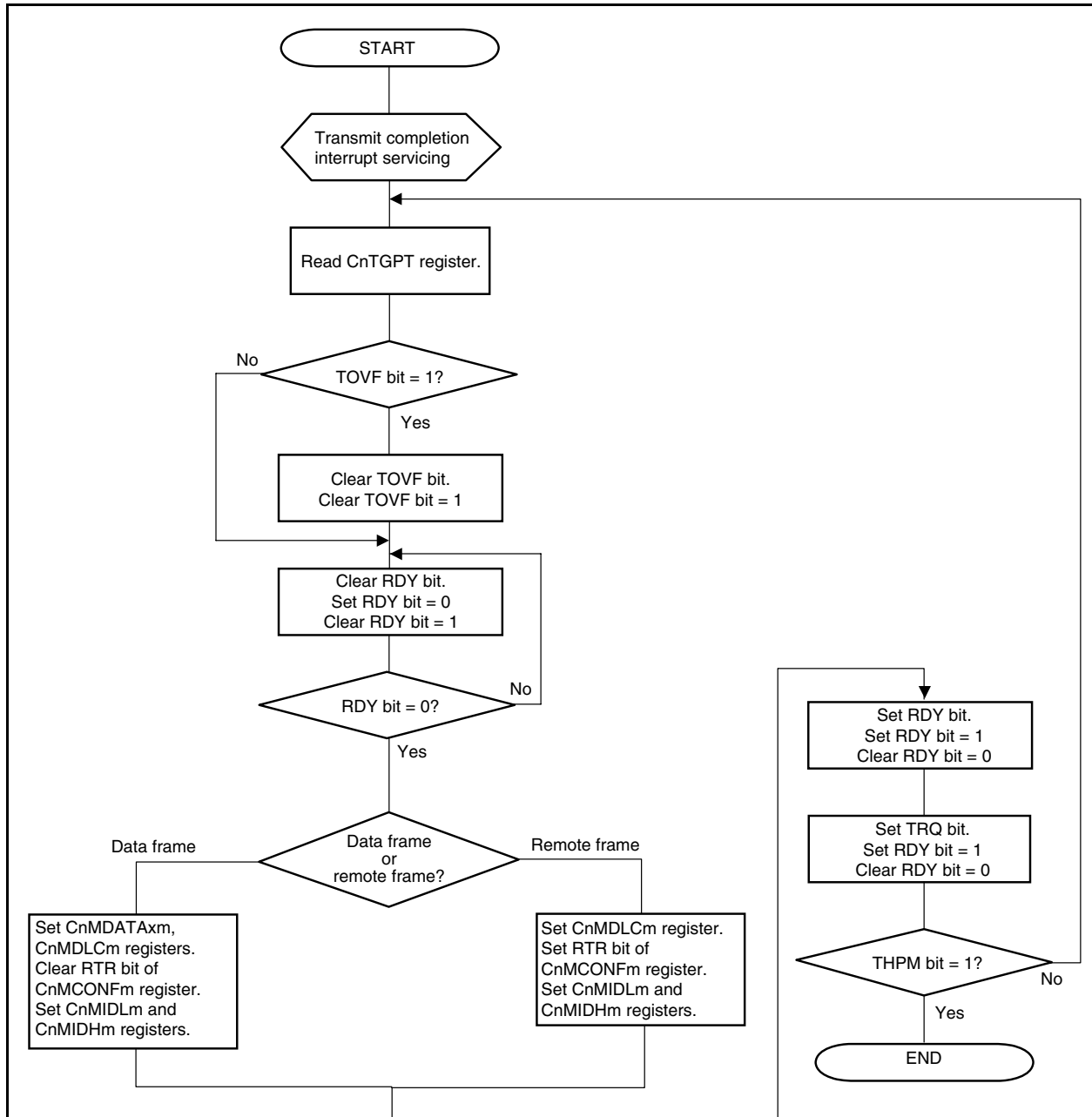
Figure 19-44. Transmission via Interrupt (Using CnTGPT Register)
