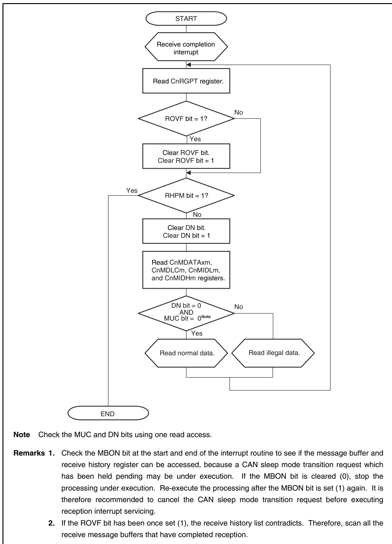
Figure 19-50. Reception via Interrupt (Using CnRGPT Register)
