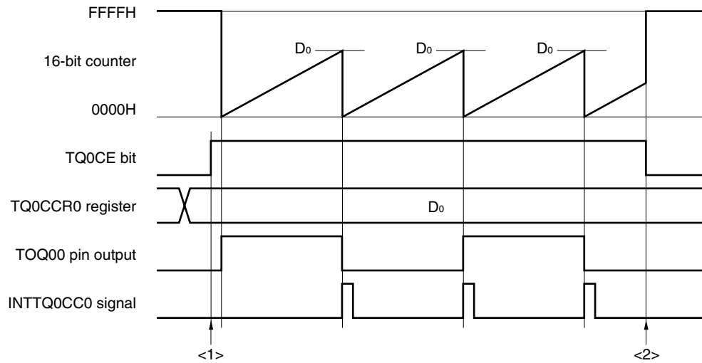
Figure 8-9. Software Processing Flow in Interval Timer Mode
