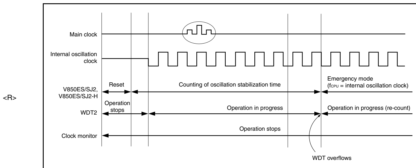
Figure 25-7. Operation After Reset Release
