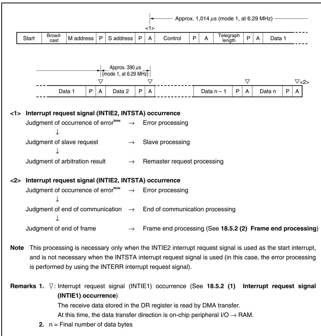
Figure 18-27. Master Reception
