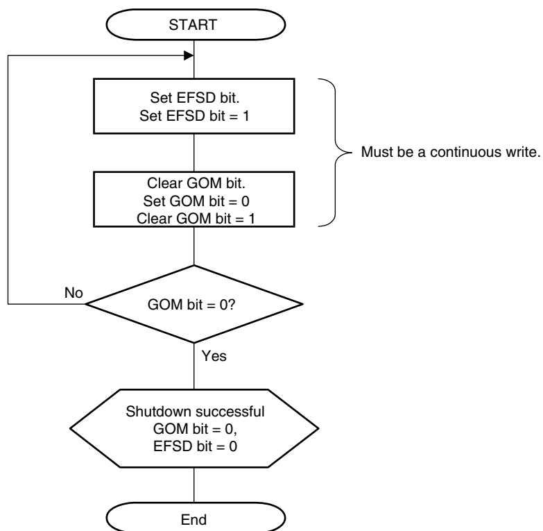
Figure 19-57. Forced Shutdown Process
