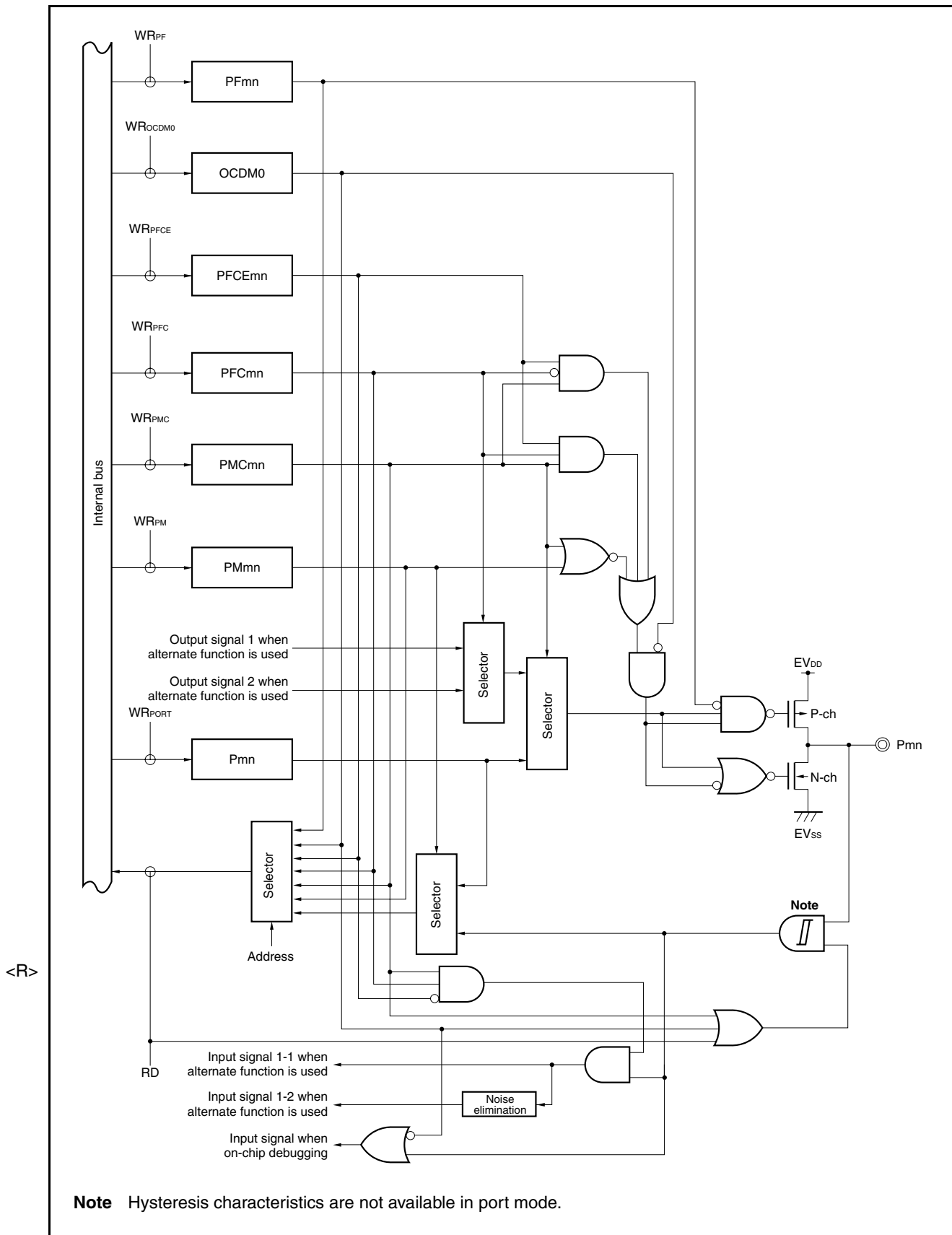
Figure 4-30. Block Diagram of Type U-6
