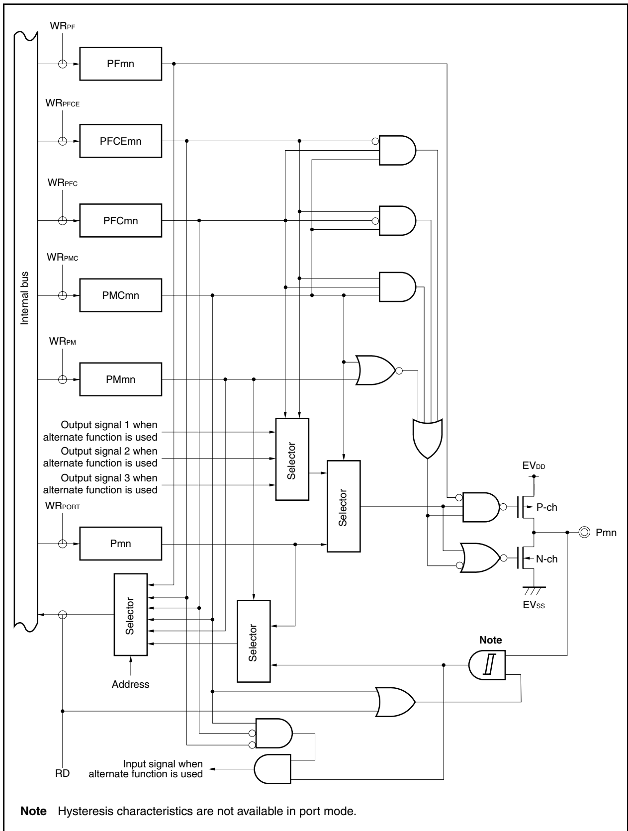
Figure 4-26. Block Diagram of Type U-2
