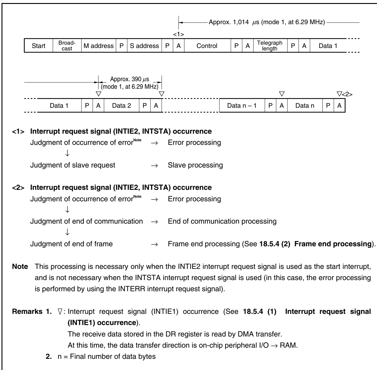
Figure 18-29. Slave Reception
