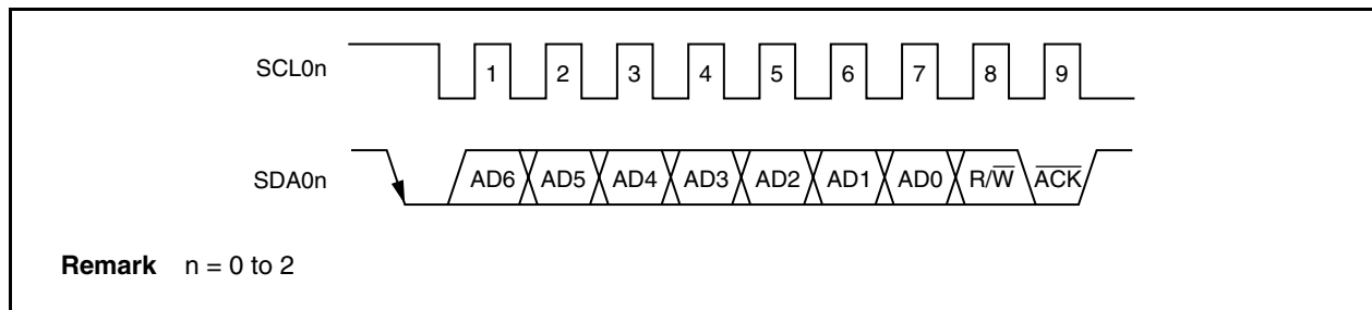
Figure 17-11. \overline{\text{ACK}}
