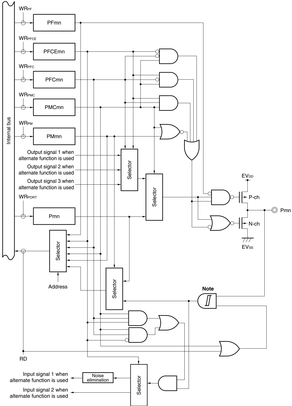
Figure 4-34. Block Diagram of Type U-10
