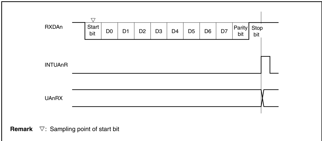
Figure 15-13. UART Reception
