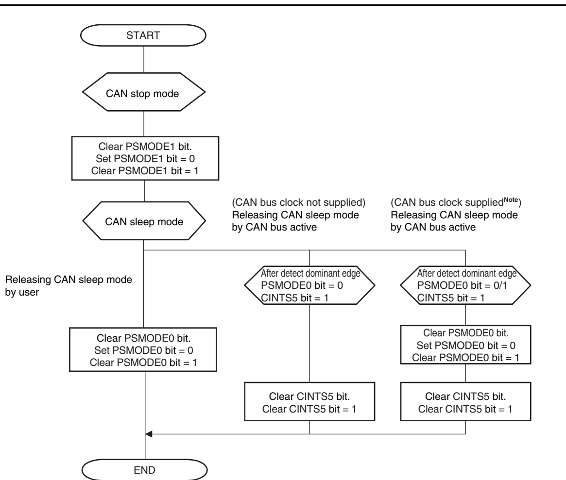
Figure 19-53. Clear CAN Sleep/Stop Mode
