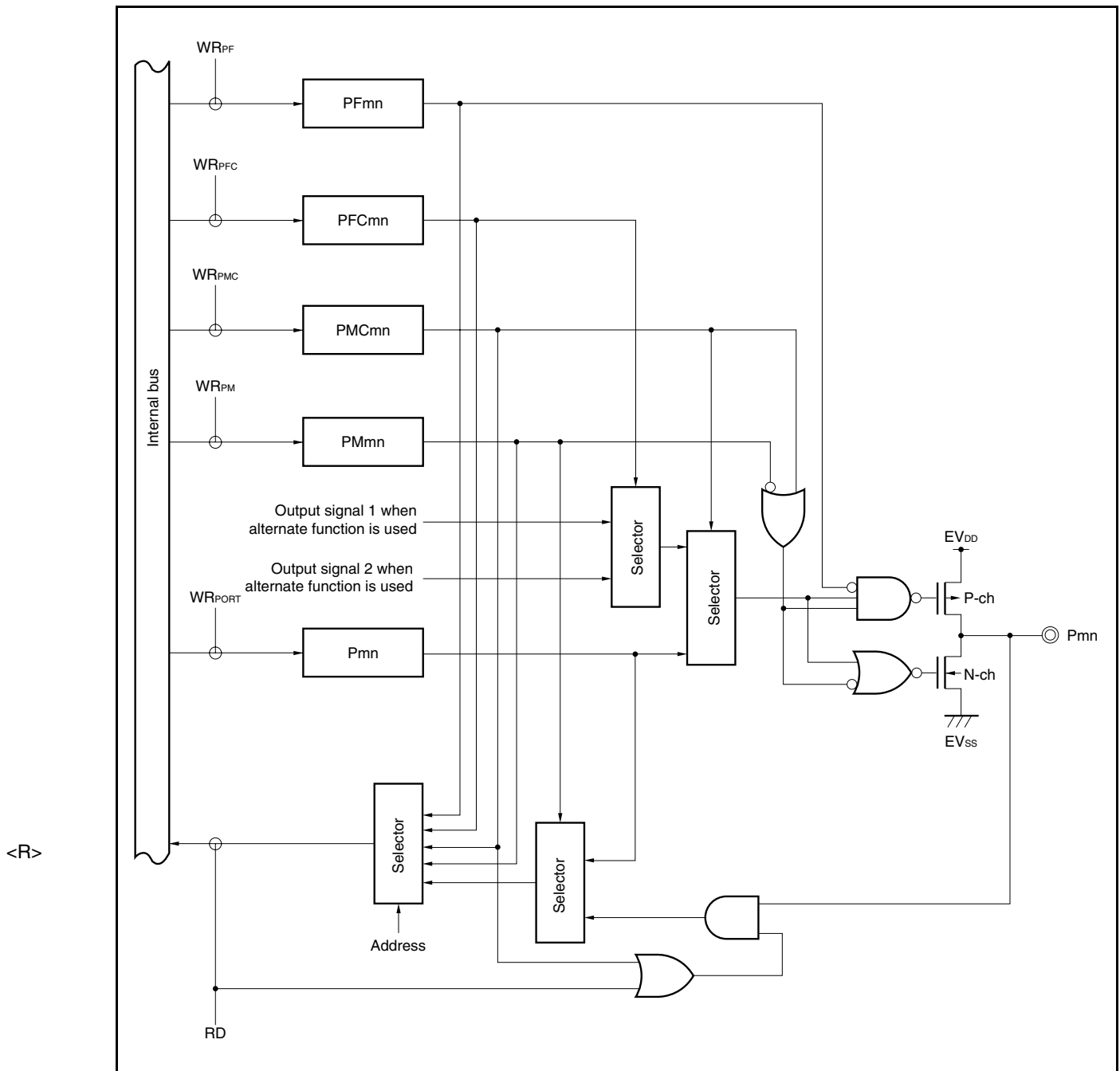
Figure 4-15. Block Diagram of Type G-3
