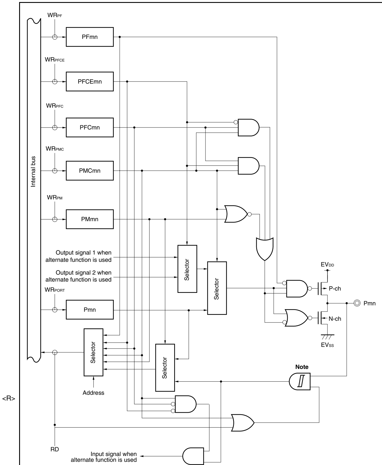
Figure 4-28. Block Diagram of Type U-4
