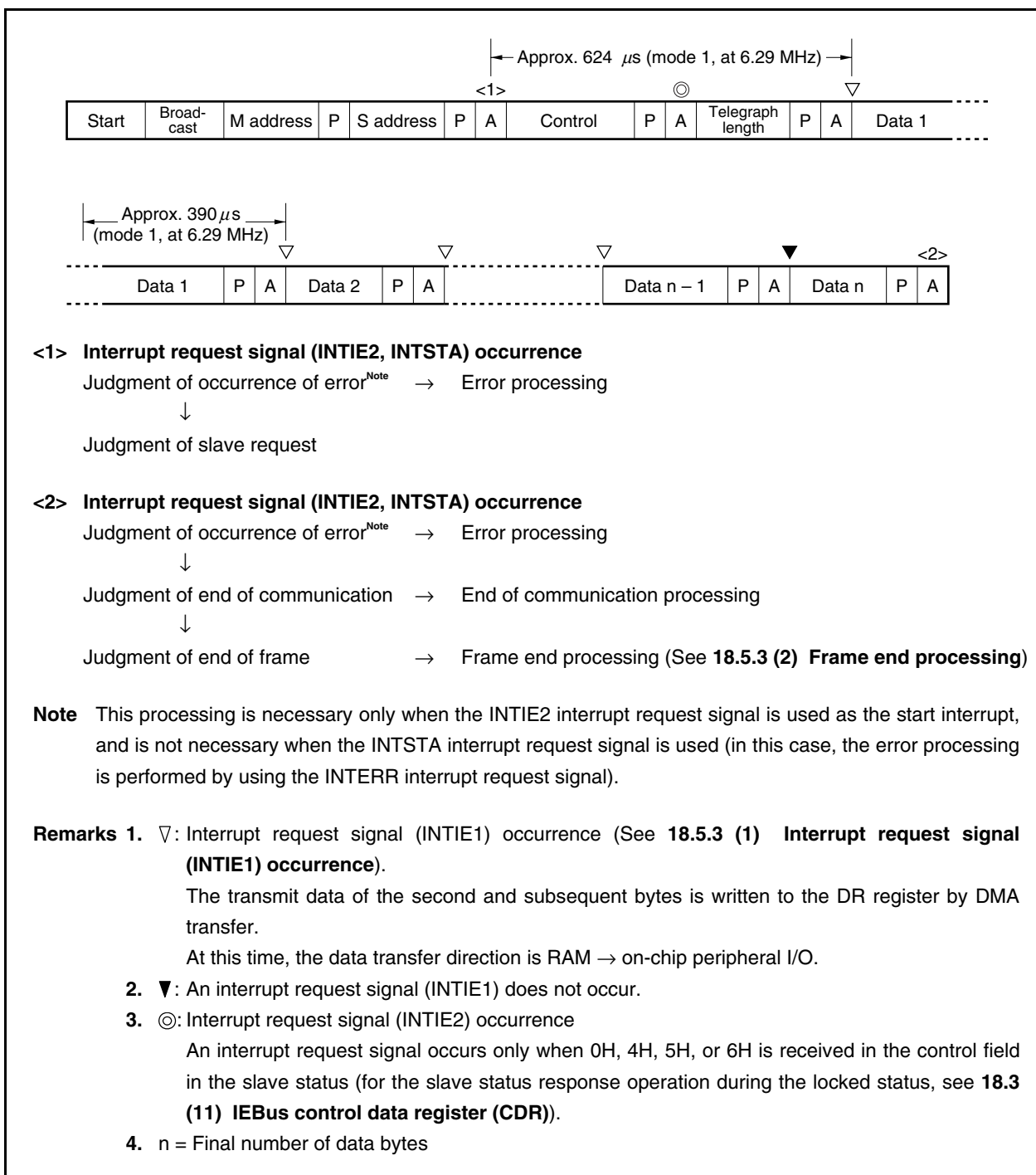
Figure 18-28. Slave Transmission
