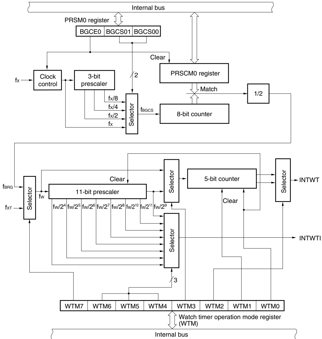
Figure 10-1. Block Diagram of Watch Timer
