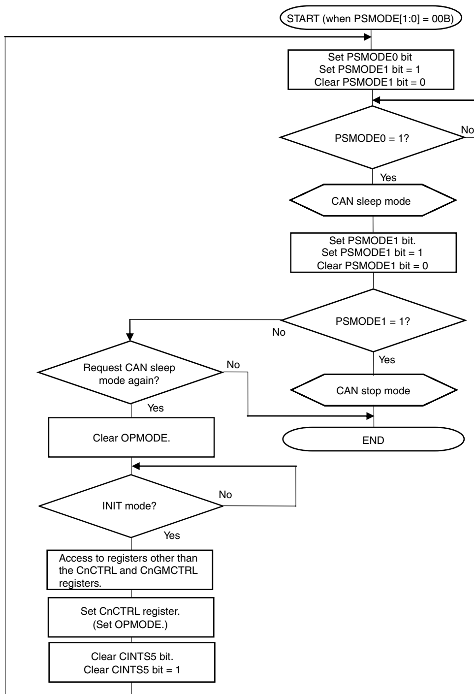
Figure 19-52. Setting CAN Sleep Mode/Stop Mode
