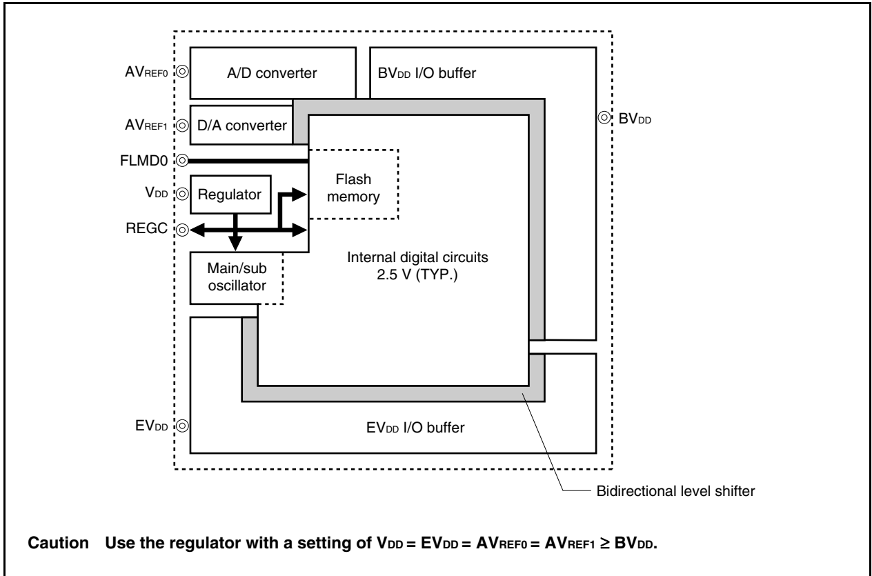
Figure 28-1. Regulator
