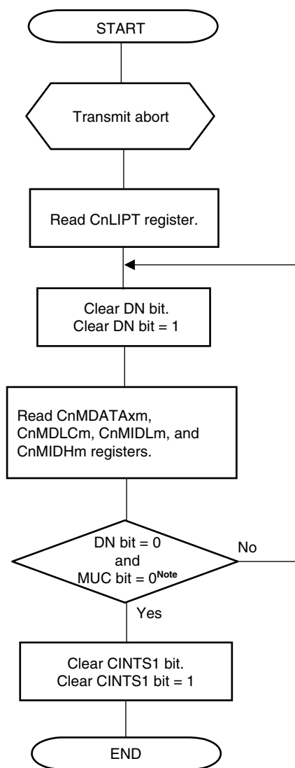
Figure 19-49. Reception via Interrupt (Using CnLIPT Register)
