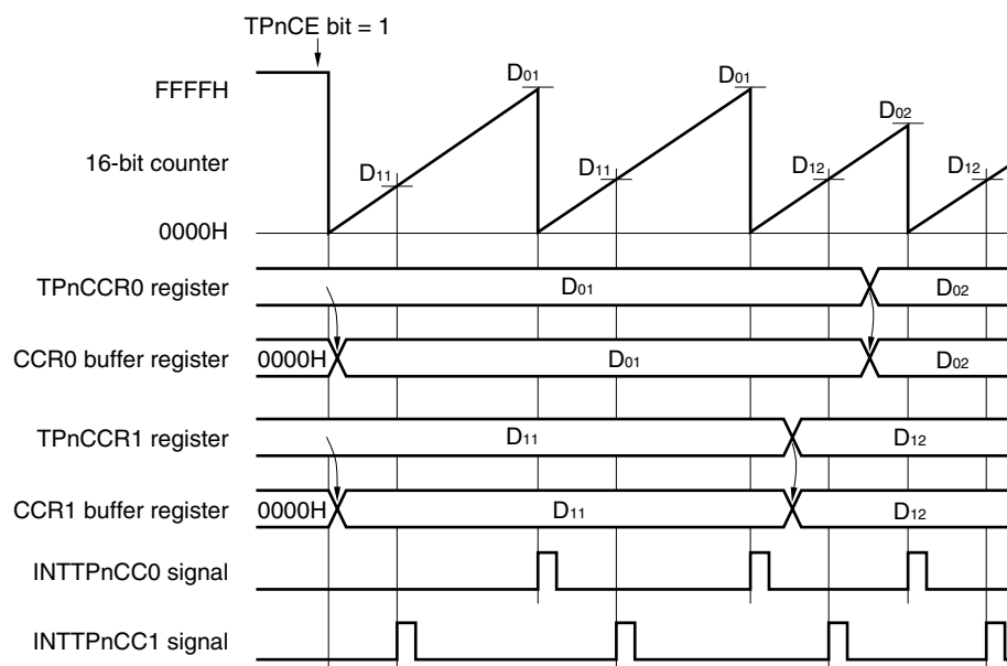
Figure 7-3. Timing of Anytime Write
