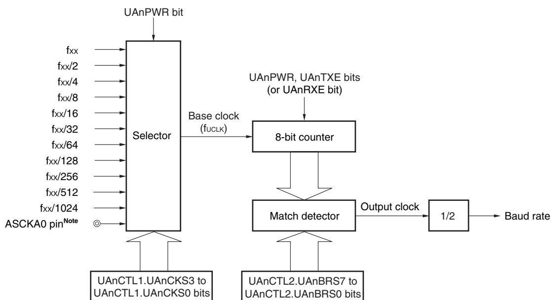
Figure 15-16. Configuration of Baud Rate Generator
