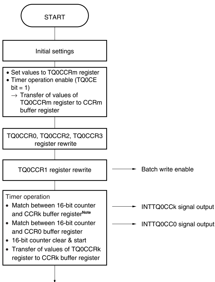
Figure 8-4. Flowchart of Basic Operation for Batch Write
