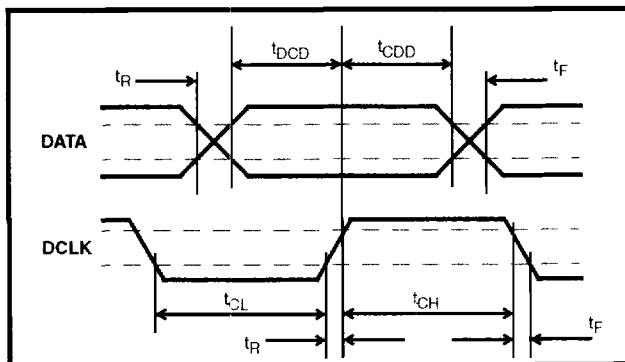
Figure 7 - DATA and DCLK Output Timing
