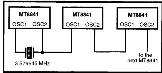
Figure 5 - Common Crystal Connection
