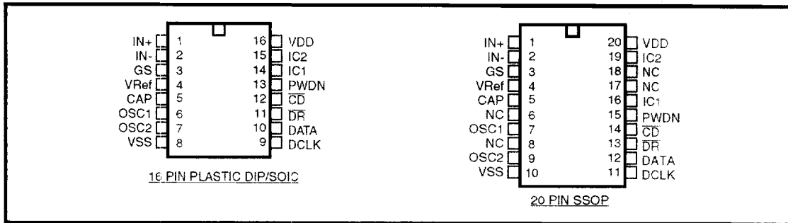
Figure 2 - Pin Connections
