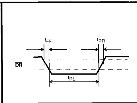
Figure 8 - \overline{DR} Output Timing
