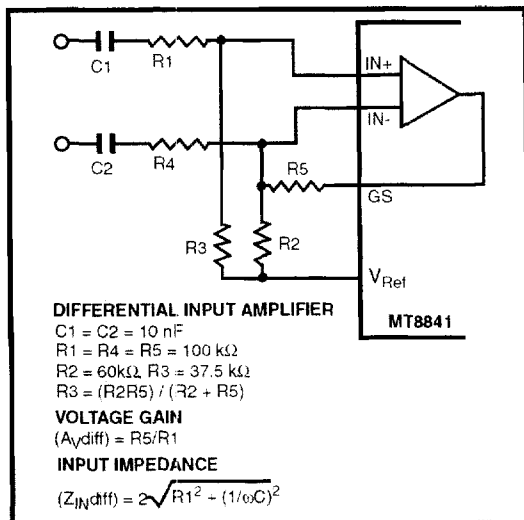
Figure 3 - Differential Input Configuration
