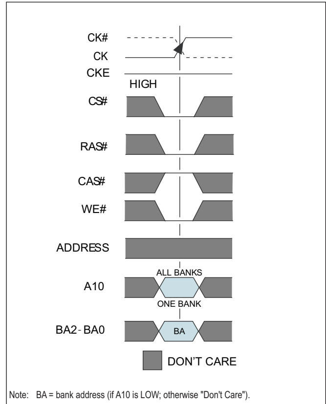
FIGURE 13 – PRECHARGE COMMAND
